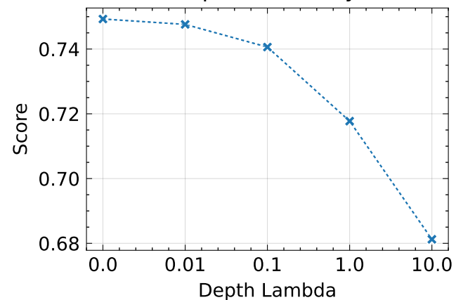
Composite Quality ↑
