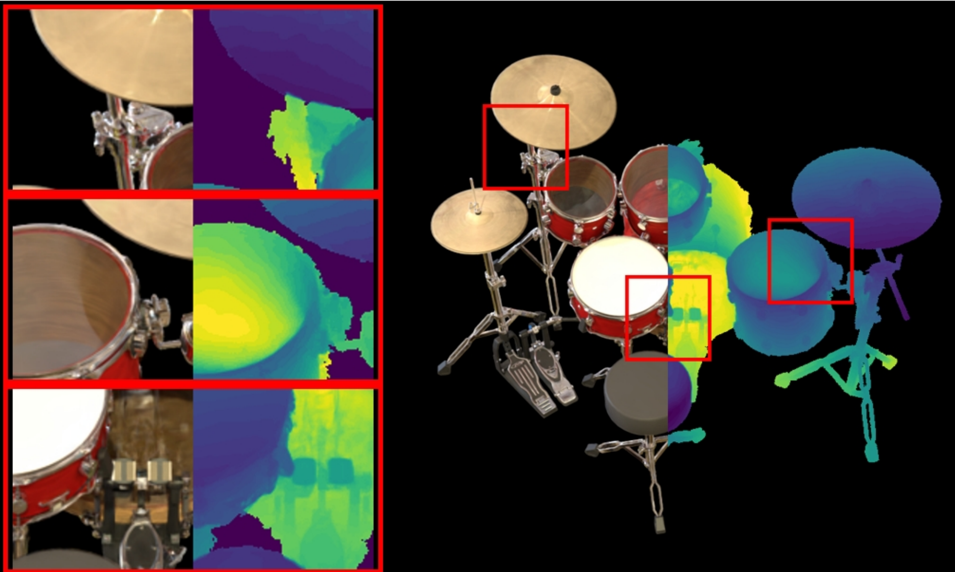
drums: VGGT | depth_lambda=0.01 PSNR: 20.85 | LPIPS: 0.0852 | SSIM: 0.8682
