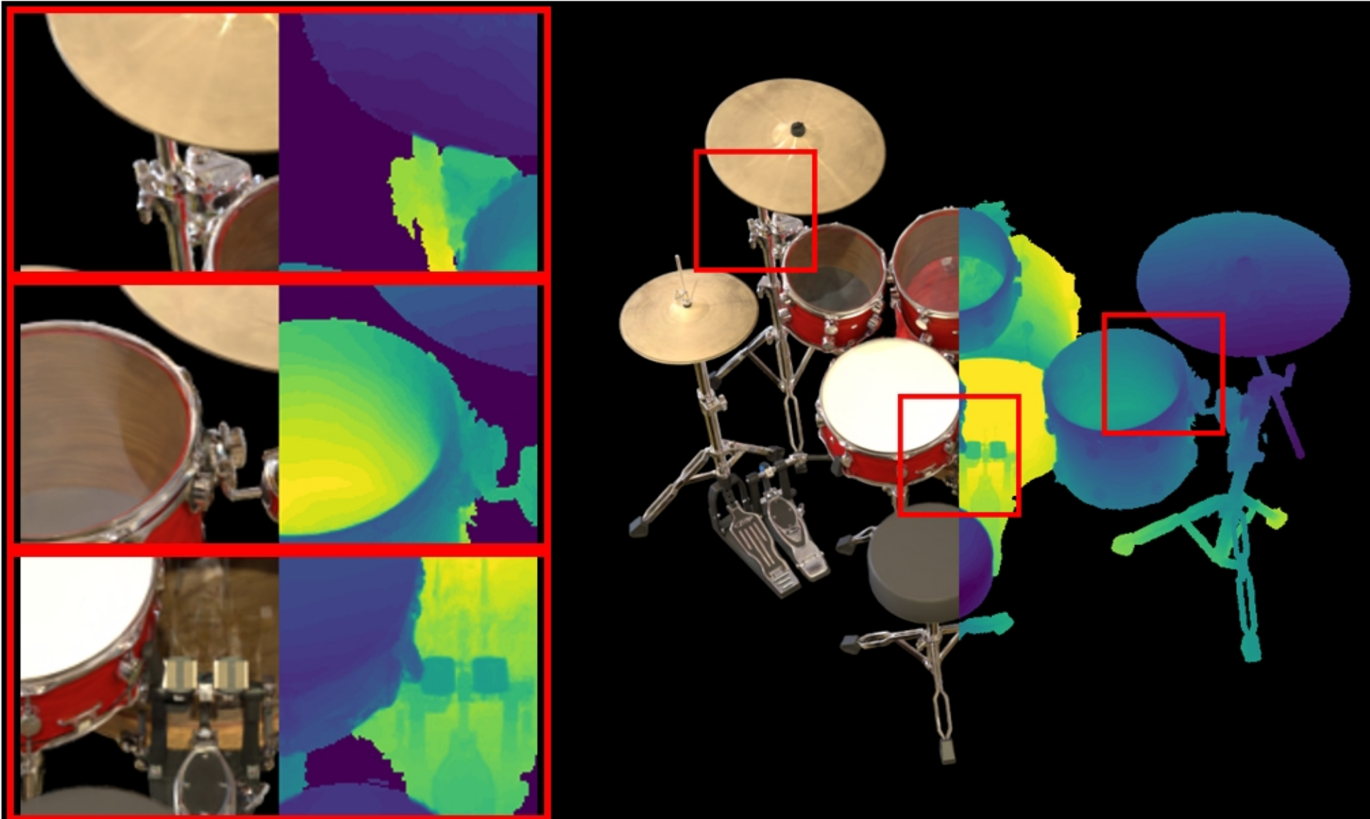
drums: VGGT | depth_lambda=0.1 PSNR: 20.65 | LPIPS: 0.0864 | SSIM: 0.8637
