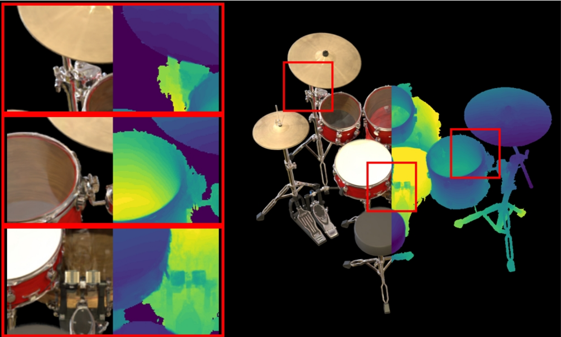
drums: VGGT | depth_lambda=1.0 PSNR: 20.01 | LPIPS: 0.0917 | SSIM: 0.8505
