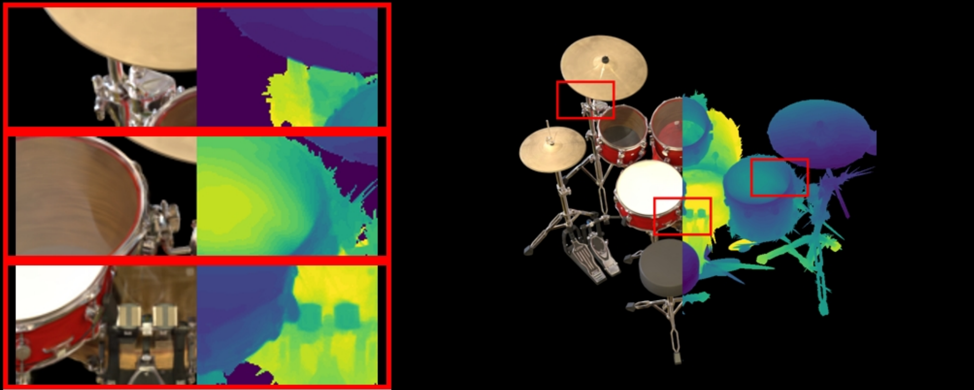
drums: COLMAP | PSNR: 22.80 | LPIPS: 0.0892 | SSIM: 0.9061
