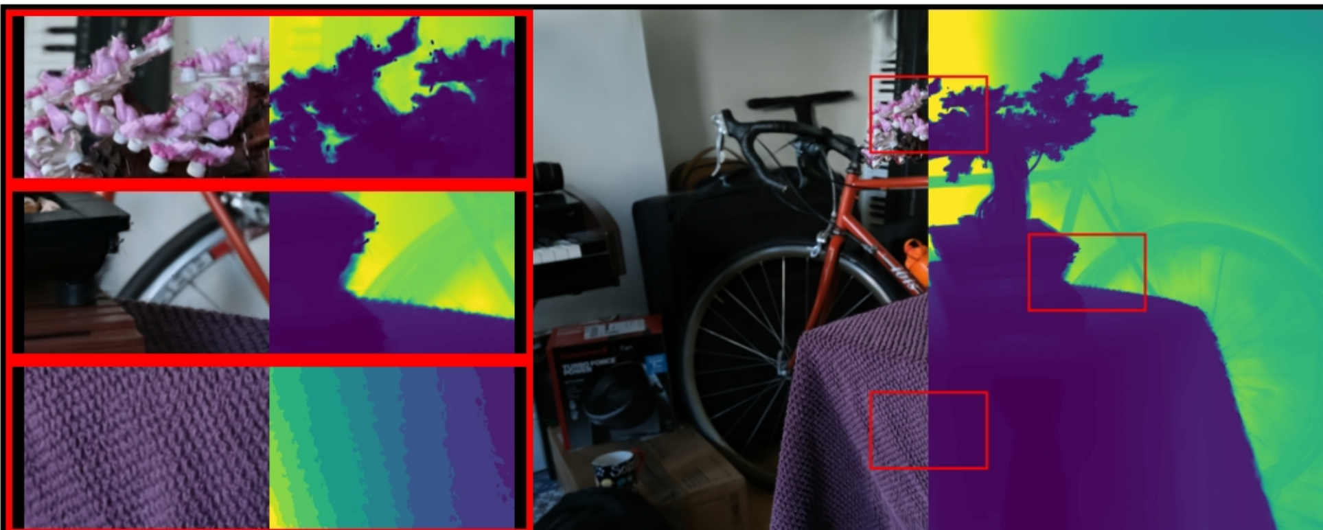
bonsai: COLMAP | points PSNR: 24.10 | LPIPS: 0.1852 | SSIM: 0.7678
