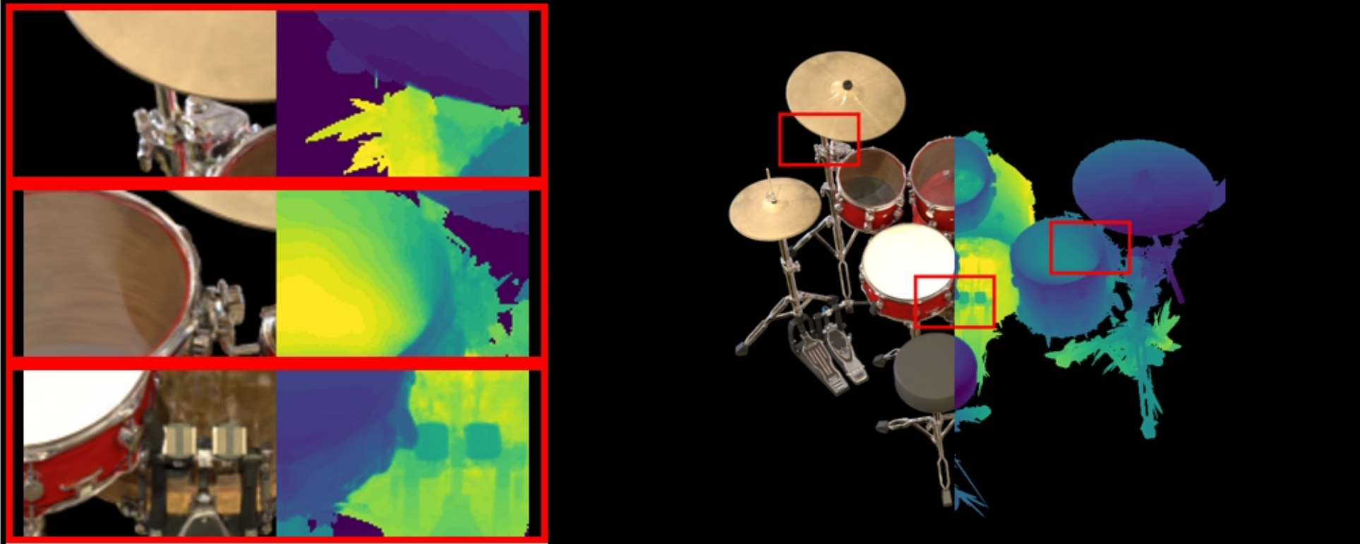
drums: VGGT | PSNR: 20.90 | LPIPS: 0.0848 | SSIM: 0.8690
