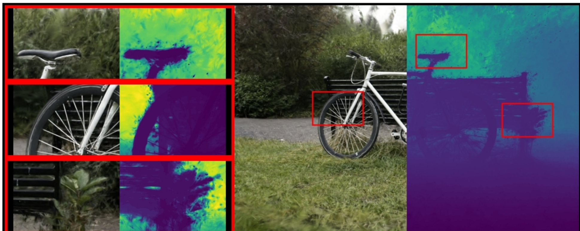
bicycle: VGGT | points PSNR: 17.41 | LPIPS: 0.3828 | SSIM: 0.2689
