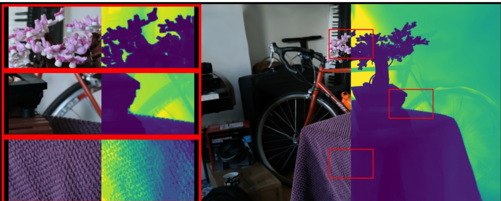
bonsai: COLMAP | PSNR: 24.65 | LPIPS: 0.1745 | SSIM: 0.7762
