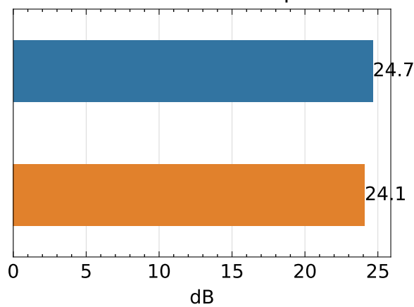
PSNR ↑ - colmap
