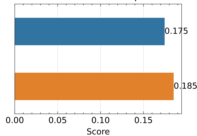
LPIPS ↓ - colmap
