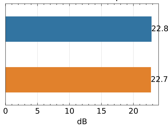
PSNR ↑ - colmap
