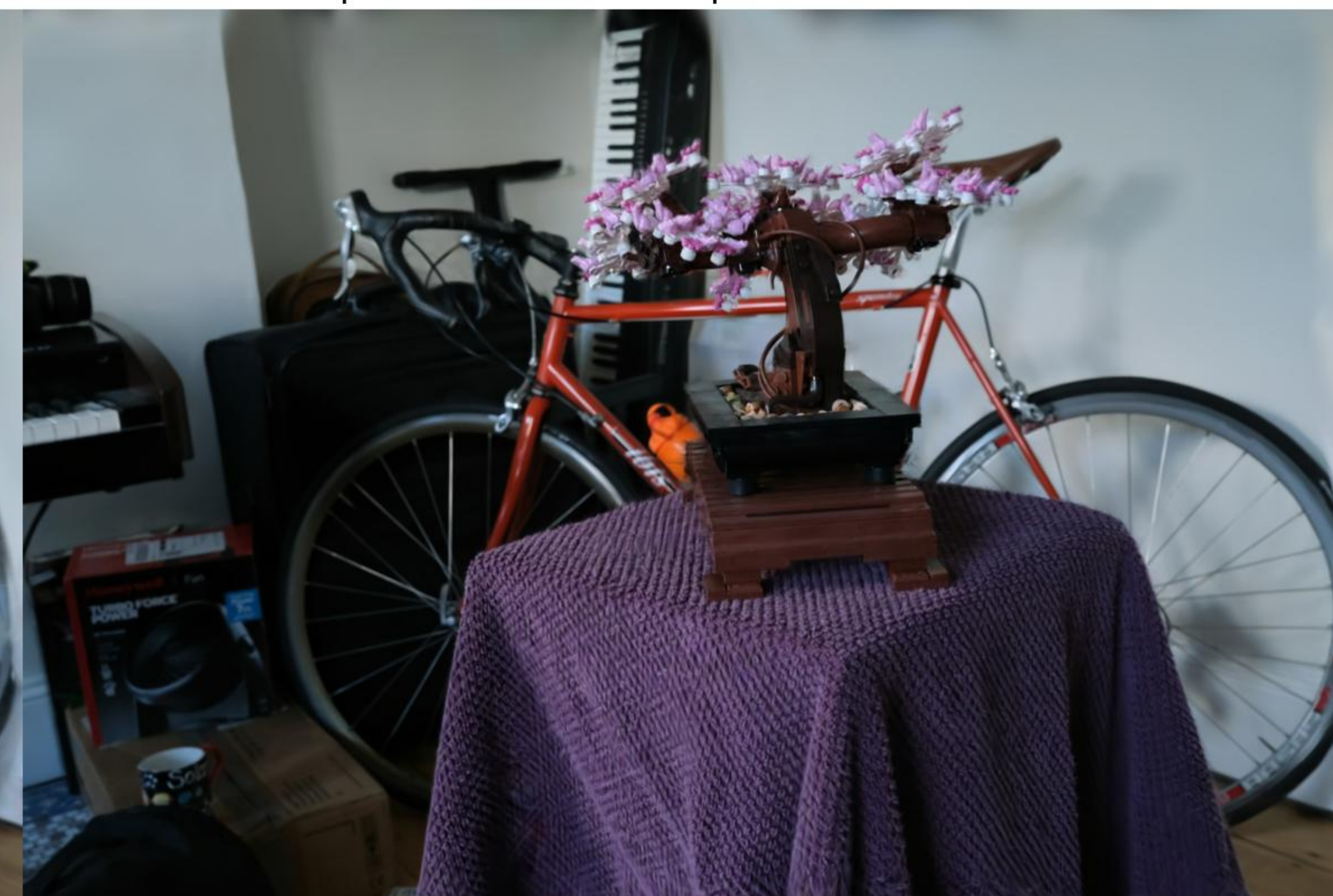
Config: VGGT | Pose Opt | num_images=40 PSNR: 17.15 | LPIPS: 0.3351 | SSIM: 0.5669
