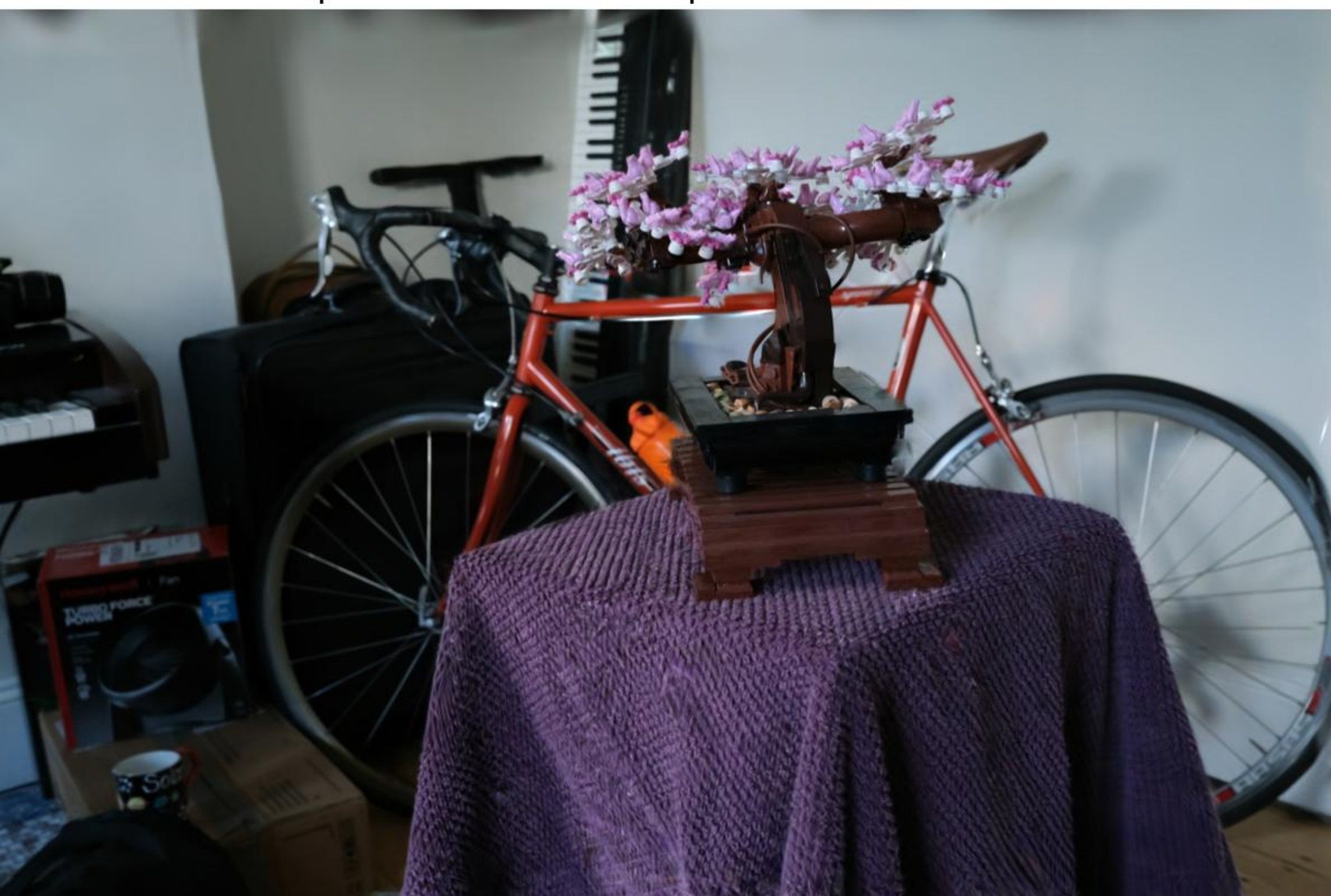
Config: VGGT | Pose Opt | num_images=20 PSNR: 18.66 | LPIPS: 0.2580 | SSIM: 0.5862
