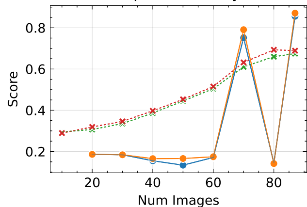
Composite Quality ↑
