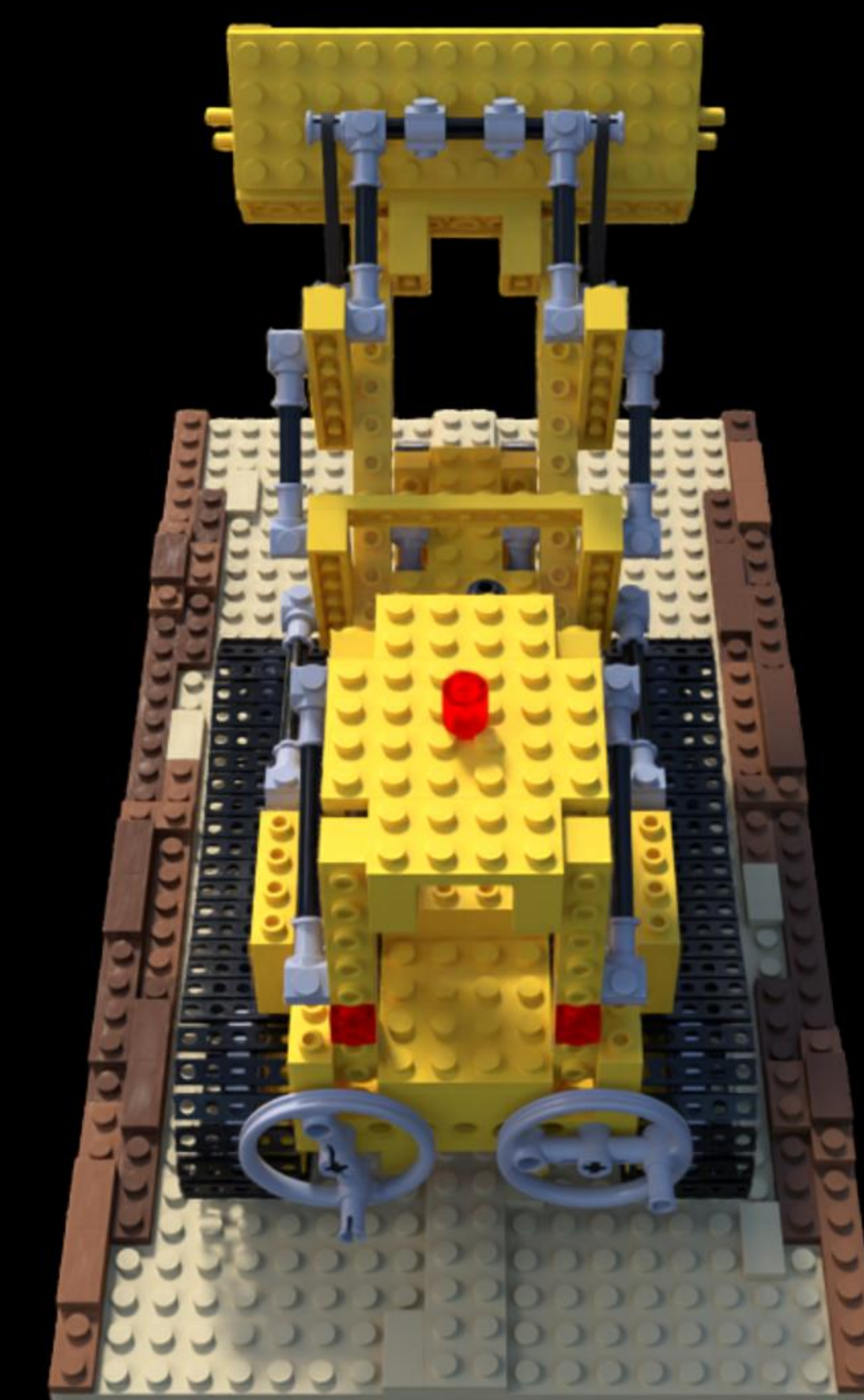
Config: VGGT | Pose Opt | num_images=87 PSNR: 25.52 | LPIPS: 0.0501 | SSIM: 0.9162
