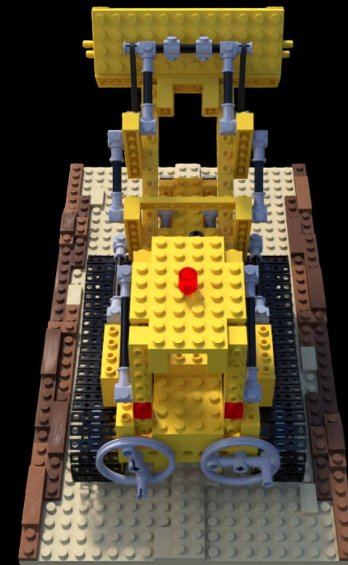
Config: COLMAP | Pose Opt | num_images=87 PSNR: 25.22 | LPIPS: 0.0518 | SSIM: 0.9104
