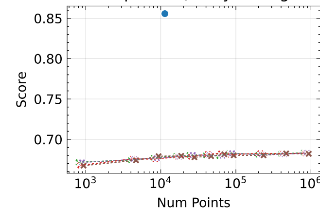
Composite Quality \uparrow - lego
