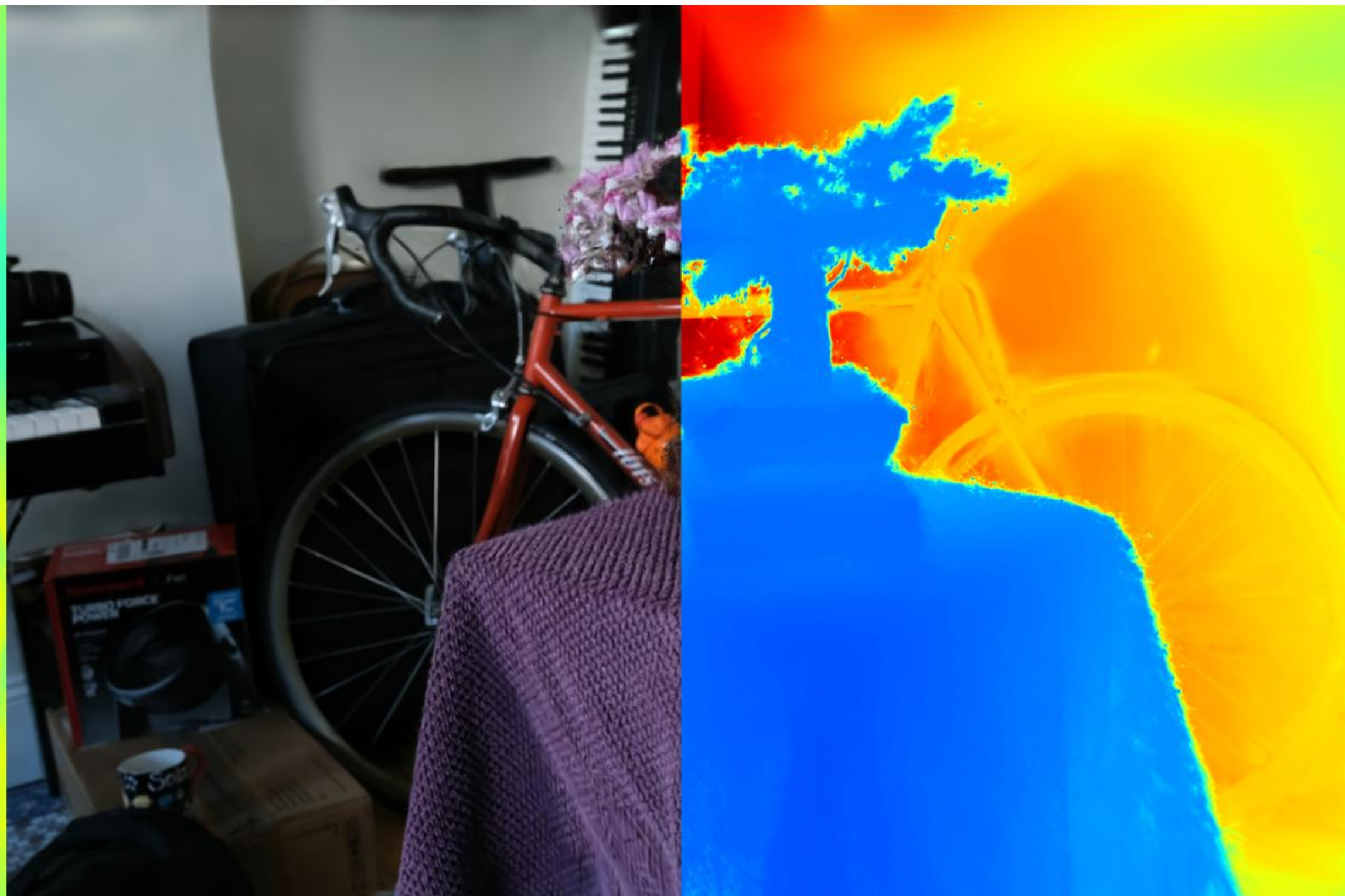
Config: VGGT | sigmoid | points | depth_lambda=1.0 PSNR: 17.23 | LPIPS: 0.3313 | SSIM: 0.5652
