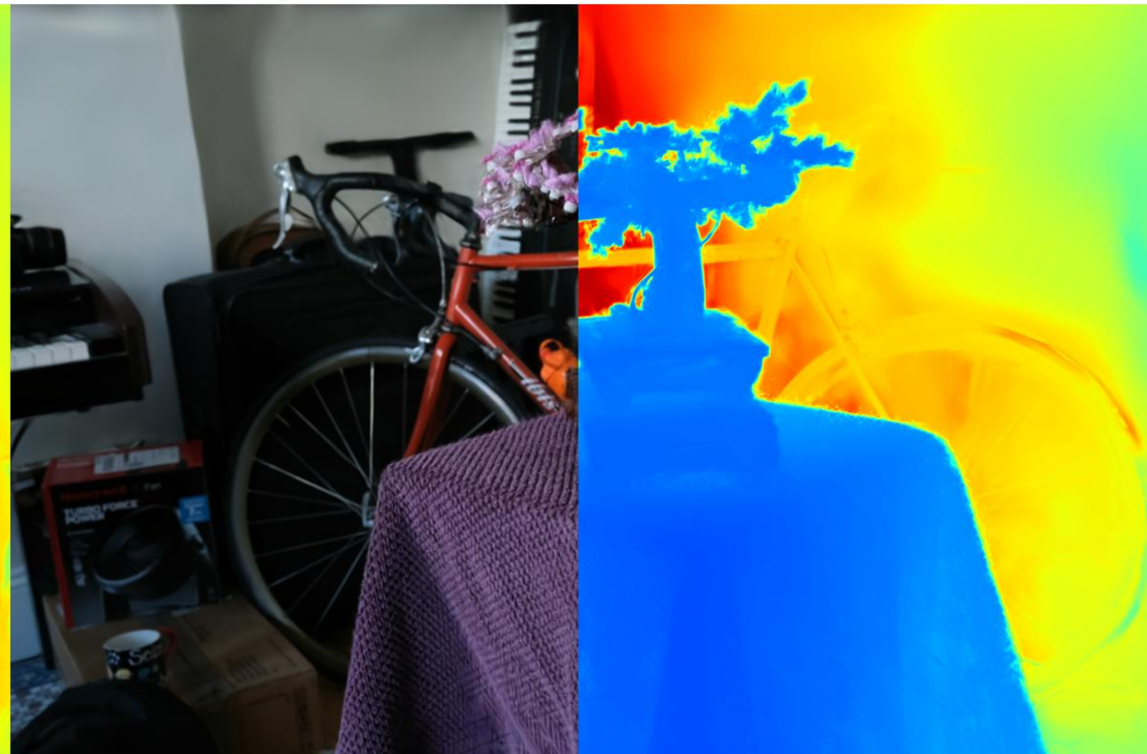
Config: VGGT | standard | points | depth_lambda=0.01 PSNR: 17.28 | LPIPS: 0.3296 | SSIM: 0.5687
