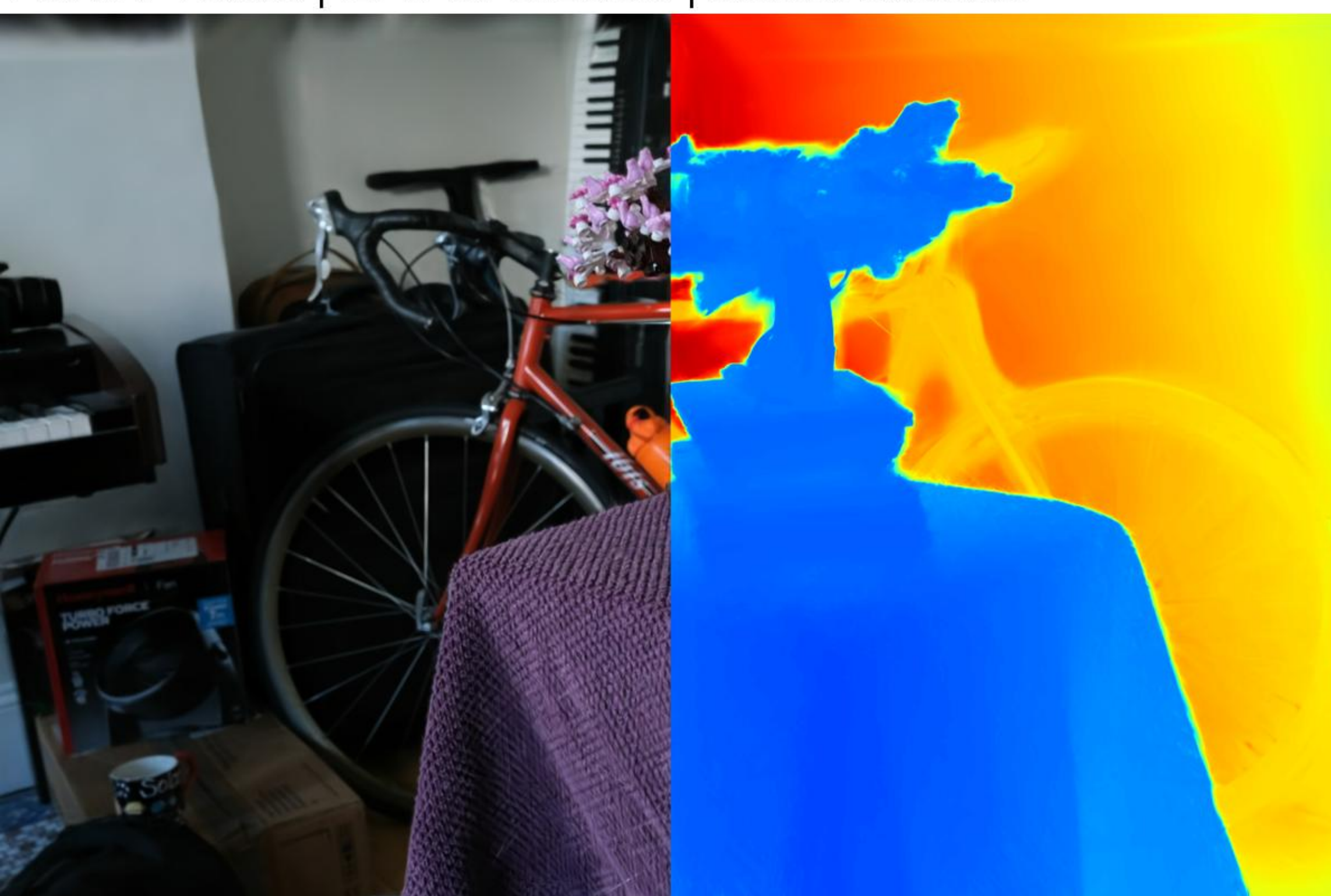
Config: VGGT | 0.1 | num_images=20 PSNR: 18.55 | LPIPS: 0.2535 | SSIM: 0.5863
