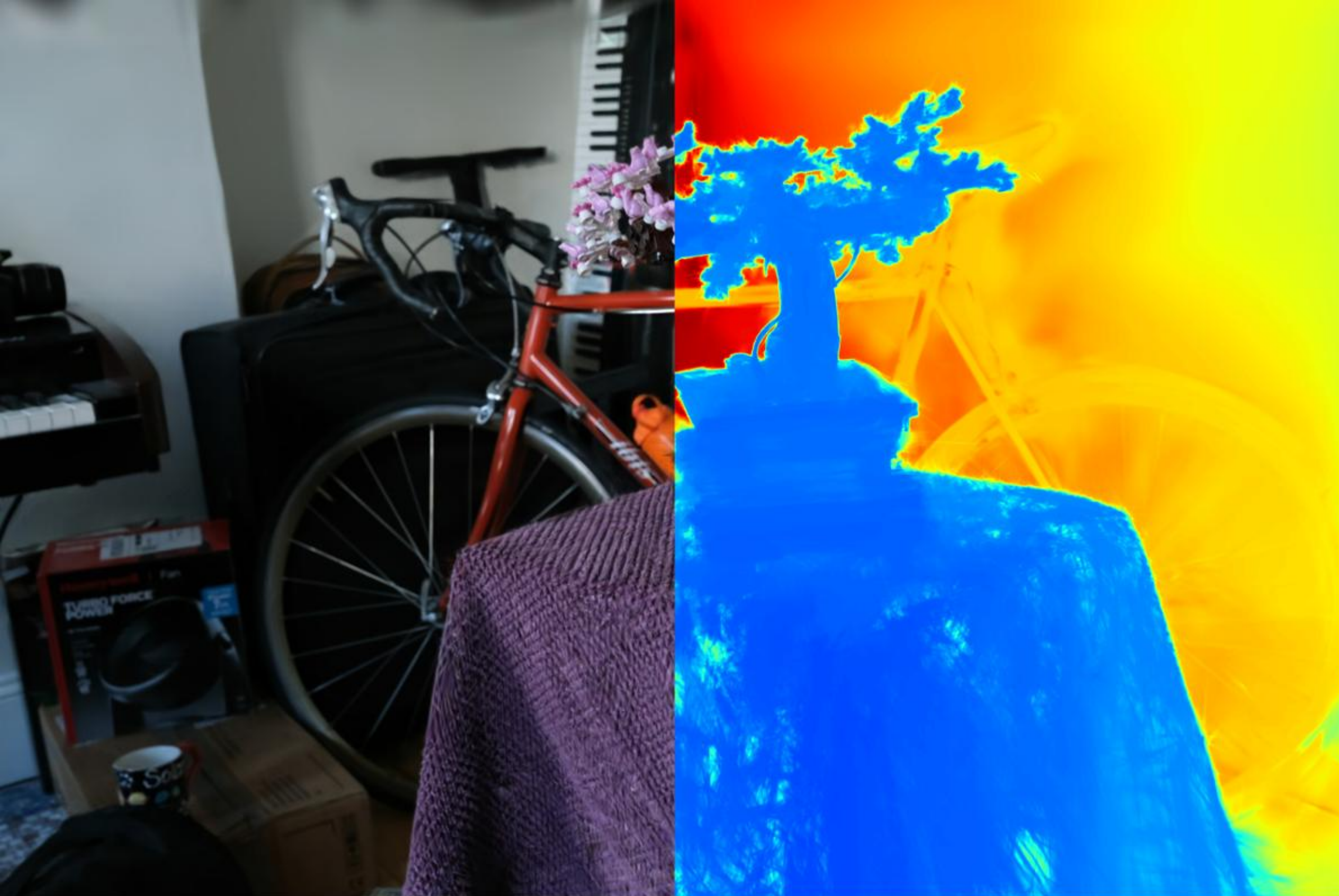
Config: VGGT | 0.0 | num_images=20 PSNR: 18.66 | LPIPS: 0.2580 | SSIM: 0.5862
