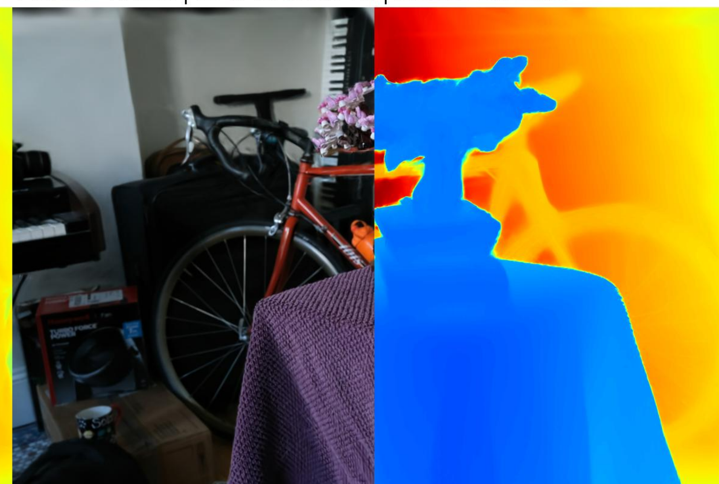
Config: VGGT | 1.0 | num_images=40 PSNR: 17.37 | LPIPS: 0.3305 | SSIM: 0.5618
