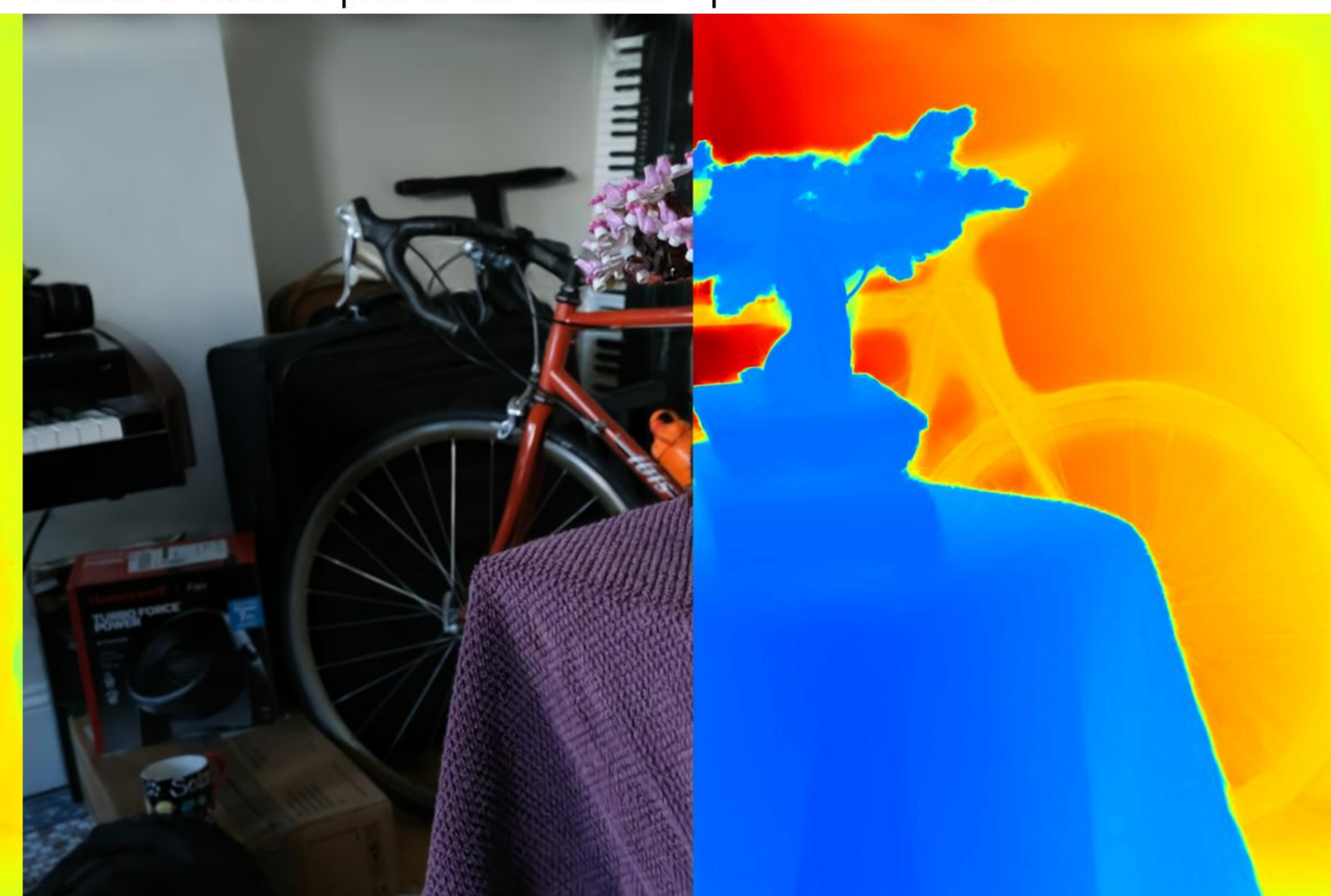
Config: VGGT | 0.1 | num_images=40 PSNR: 17.29 | LPIPS: 0.3219 | SSIM: 0.5586
