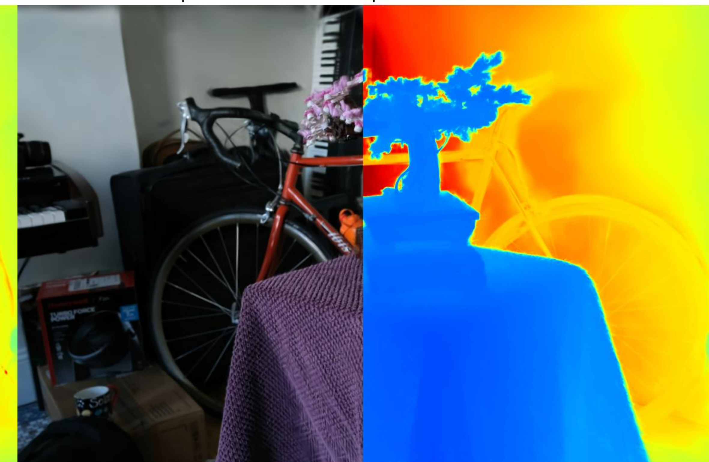
Config: VGGT | 0.01 | num_images=100 PSNR: 17.19 | LPIPS: 0.3381 | SSIM: 0.5663
