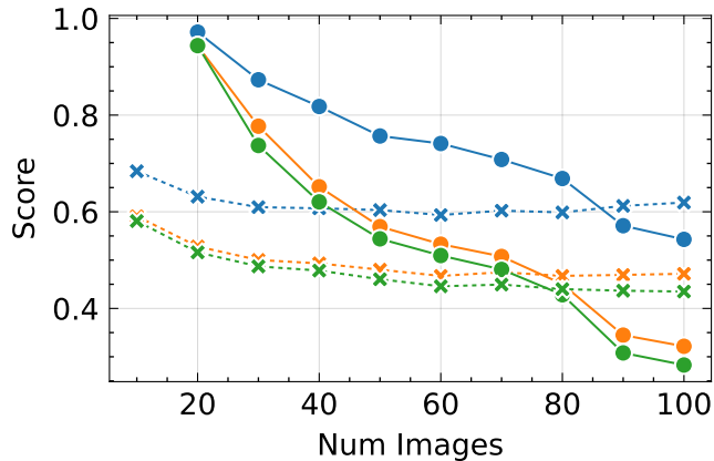
LPIPS \downarrow
