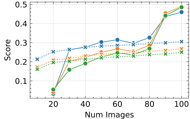
SSIM \uparrow
