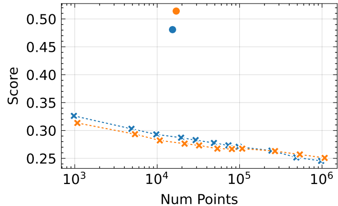
SSIM \uparrow
