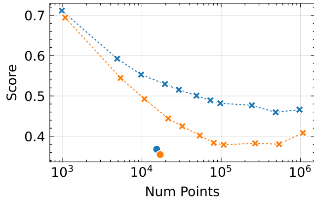
LPIPS \downarrow
