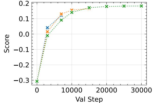
Composite Quality ↑
