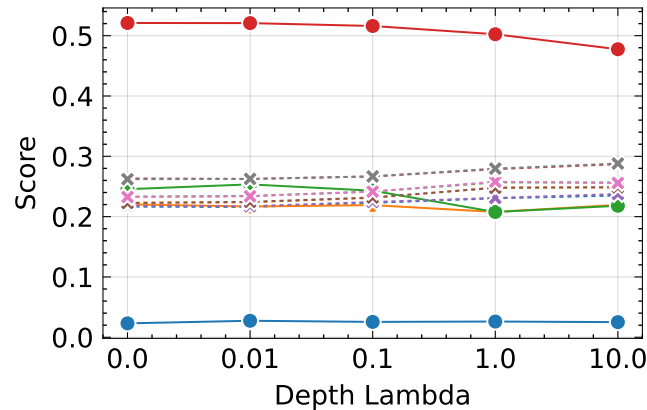
SSIM \uparrow
