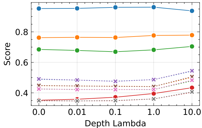
LPIPS \downarrow
