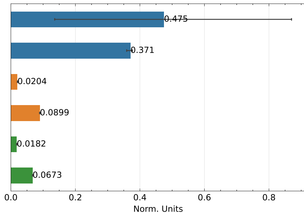
Composite Quality ↑
