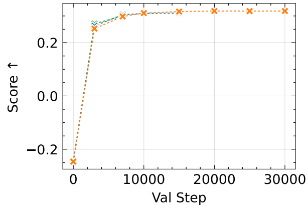
Composite Quality
