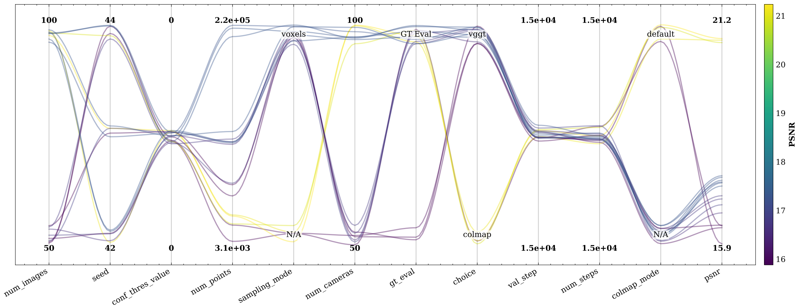
Test for dataset types - Parallel Coordinates
