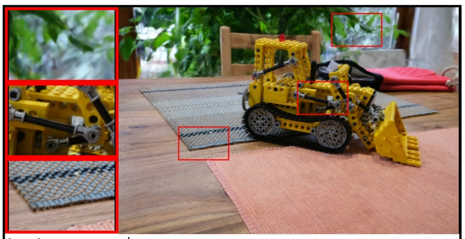
kitchen: VGGT | num_images=70 PSNR: 19.22 | LPIPS: 0.2482 | SSIM: 0.4437
