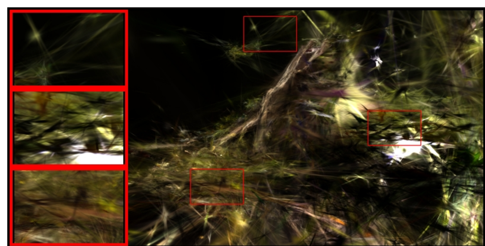
stump: COLMAP | num_images=40 PSNR: 14.15 | LPIPS: 0.6600 | SSIM: 0.3184
