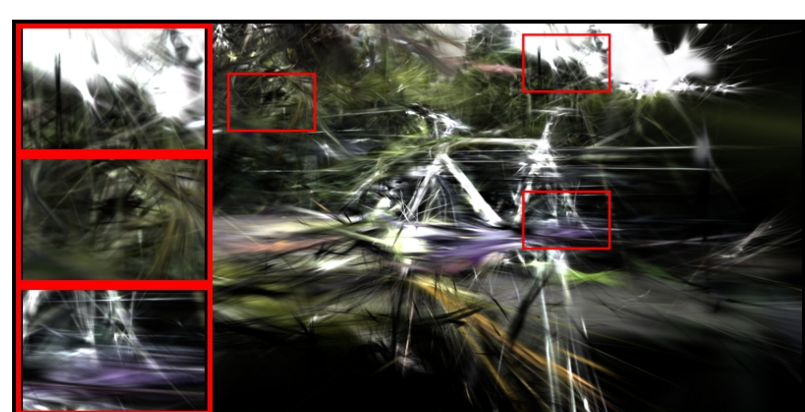
bicycle: COLMAP | num_images=30 PSNR: 12.06 | LPIPS: 0.7755 | SSIM: 0.1813
