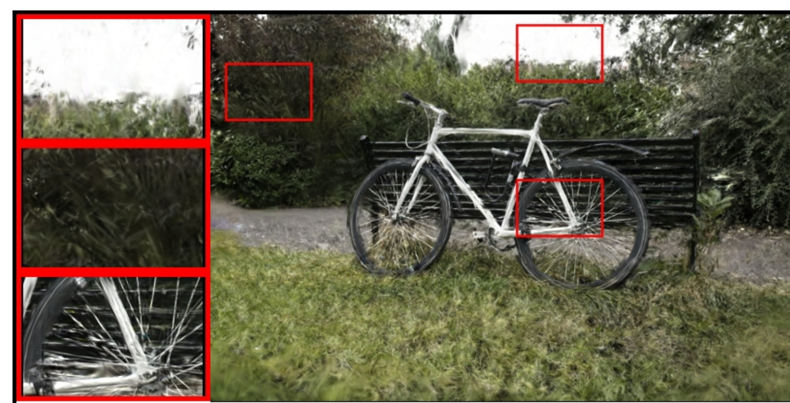
bicycle: VGGT | num_images=40 PSNR: 15.95 | LPIPS: 0.4716 | SSIM: 0.2070
