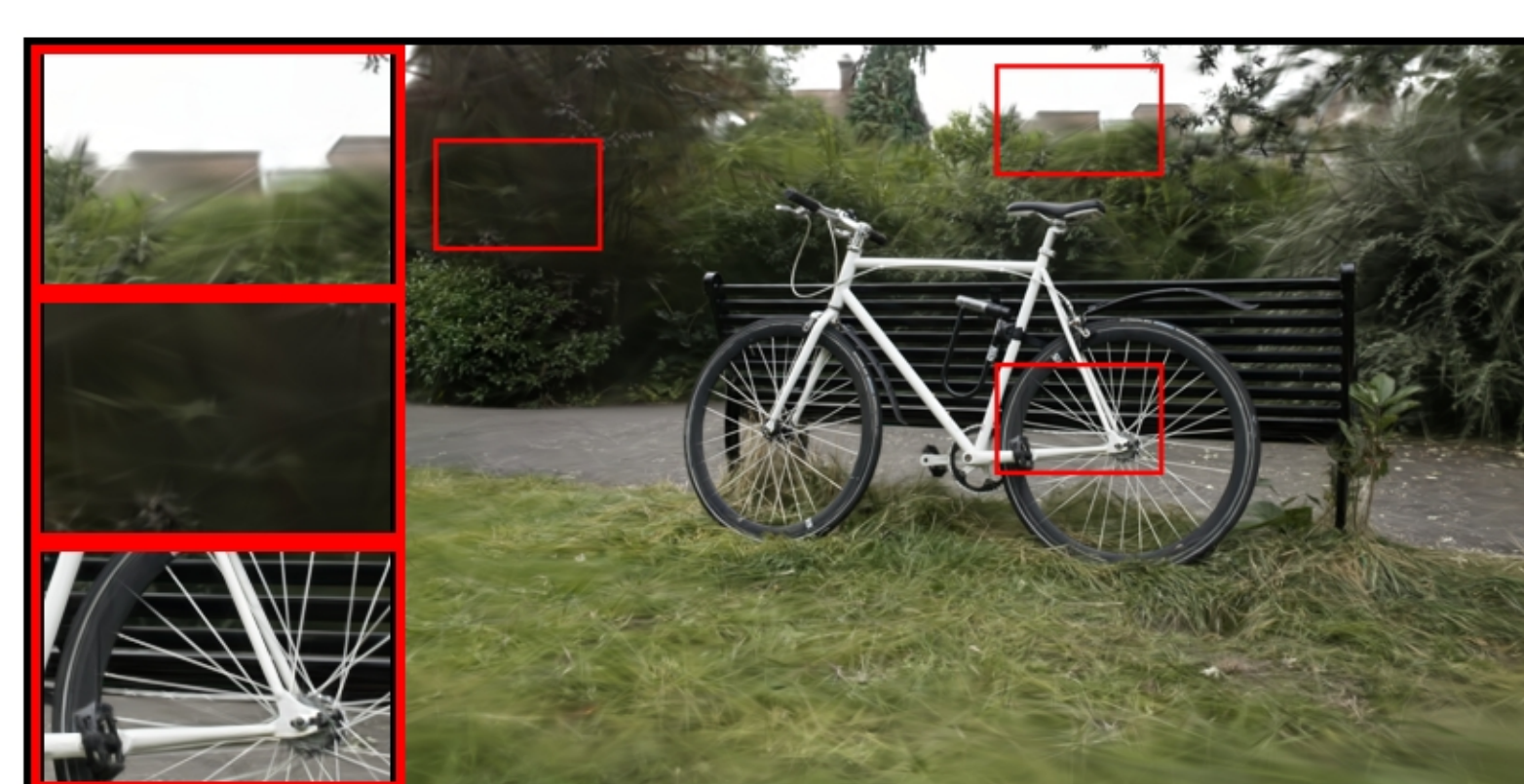
bicycle: COLMAP | num_images=100 PSNR: 21.33 | LPIPS: 0.3638 | SSIM: 0.4795
