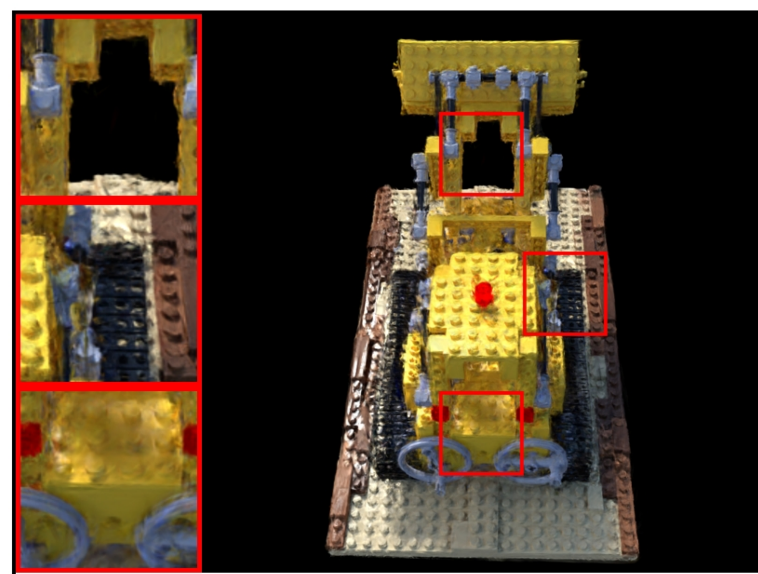
lego: VGGT | num_images=40 PSNR: 14.38 | LPIPS: 0.2763 | SSIM: 0.6544
