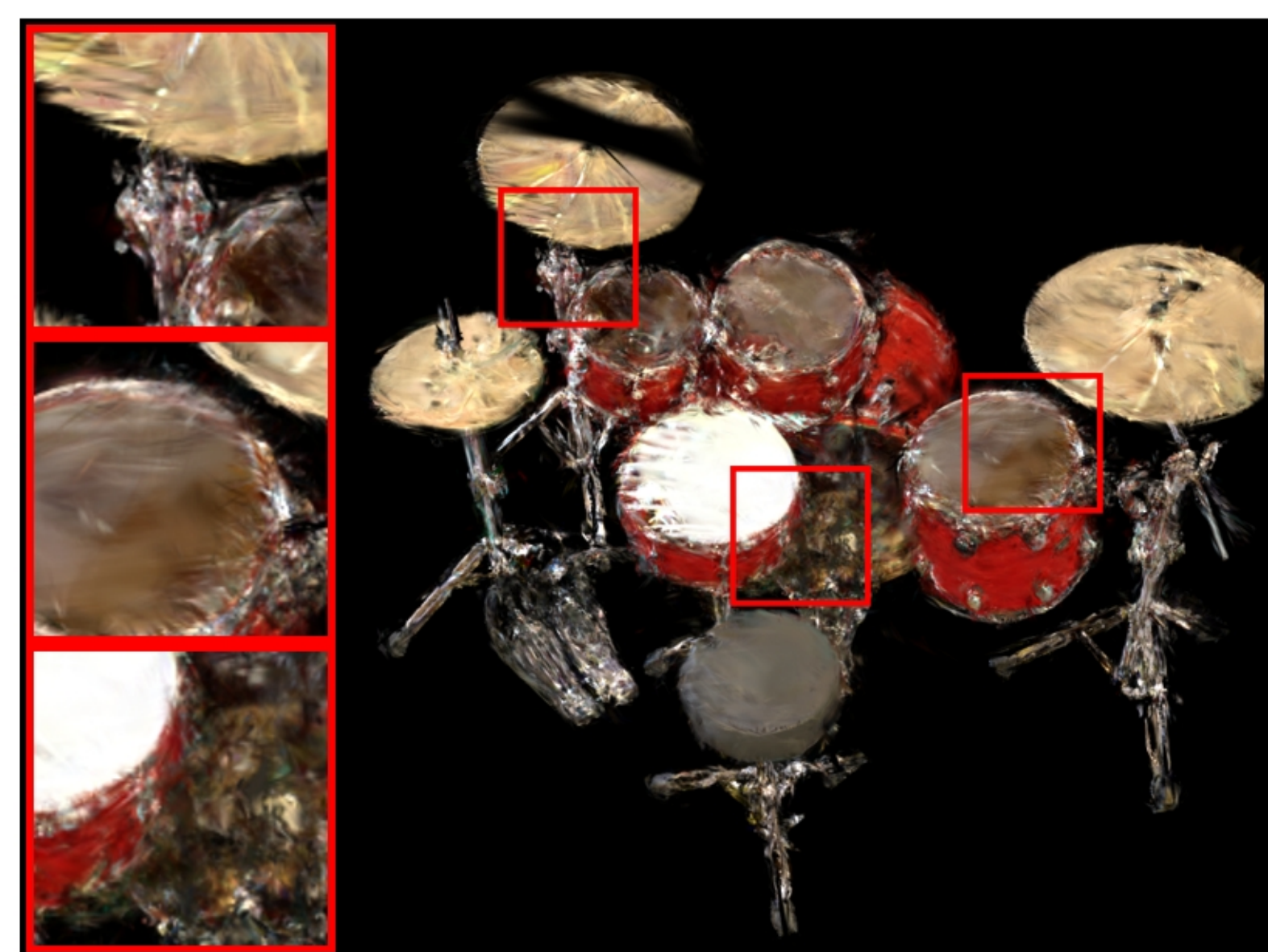
drums: VGGT | num_images=30 PSNR: 13.97 | LPIPS: 0.2957 | SSIM: 0.6801
