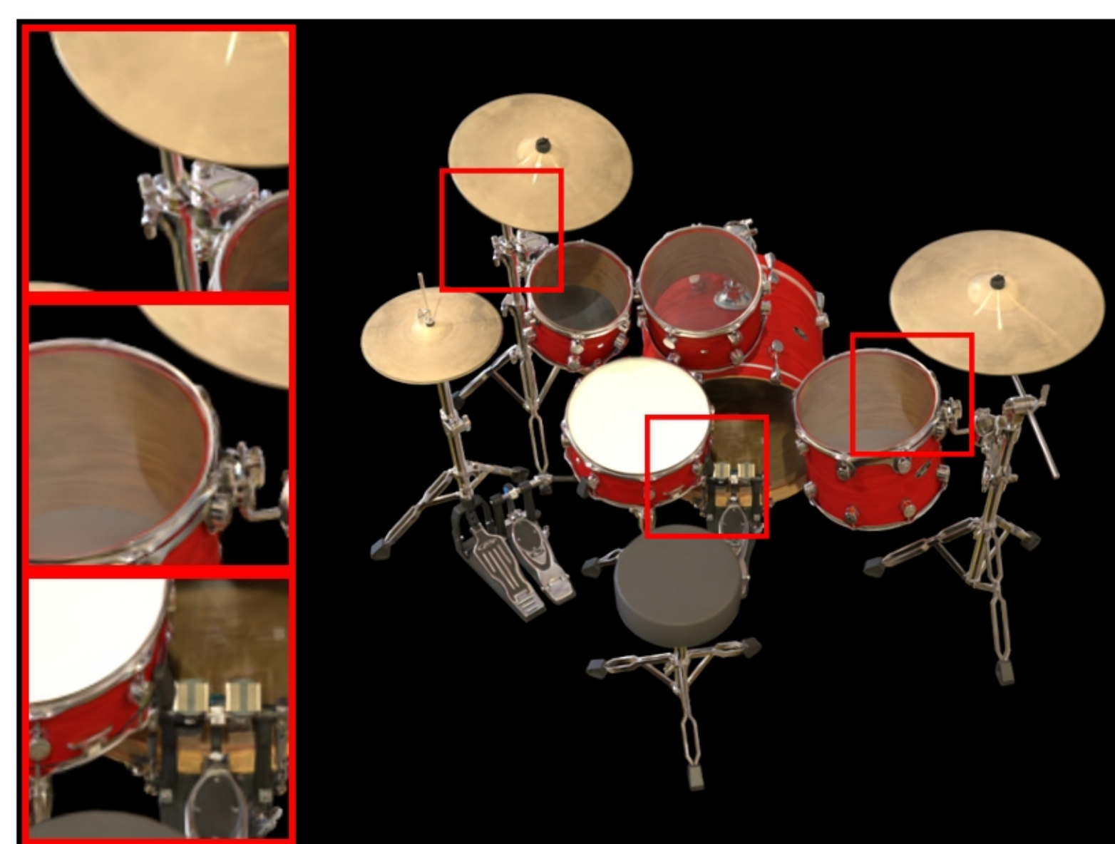
drums: COLMAP | num_images=87 PSNR: 22.47 | LPIPS: 0.0934 | SSIM: 0.8989
