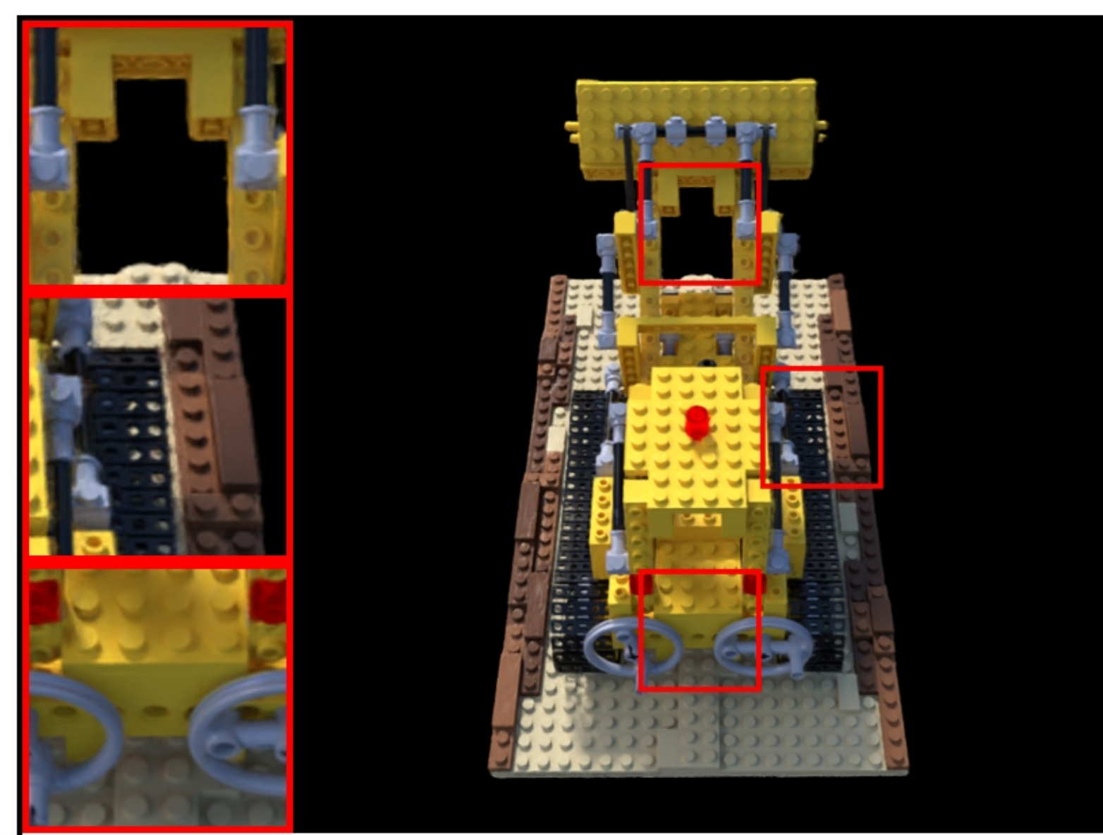
lego: VGGT | num_images=70 PSNR: 18.46 | LPIPS: 0.1258 | SSIM: 0.7529
