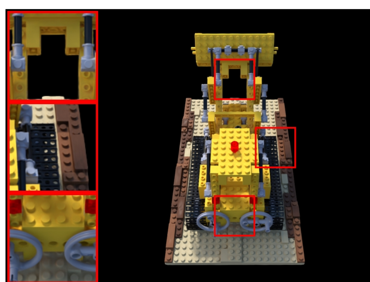
lego: COLMAP | num_images=87 PSNR: 24.95 | LPIPS: 0.0578 | SSIM: 0.8942
