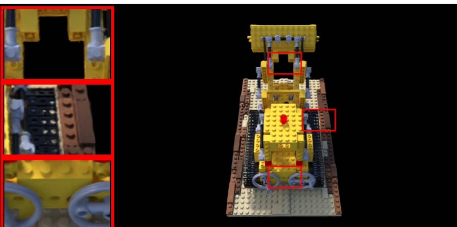
lego: VGGT | voxels | num_points=87000 PSNR: 20.56 | LPIPS: 0.0959 | SSIM: 0.7731
