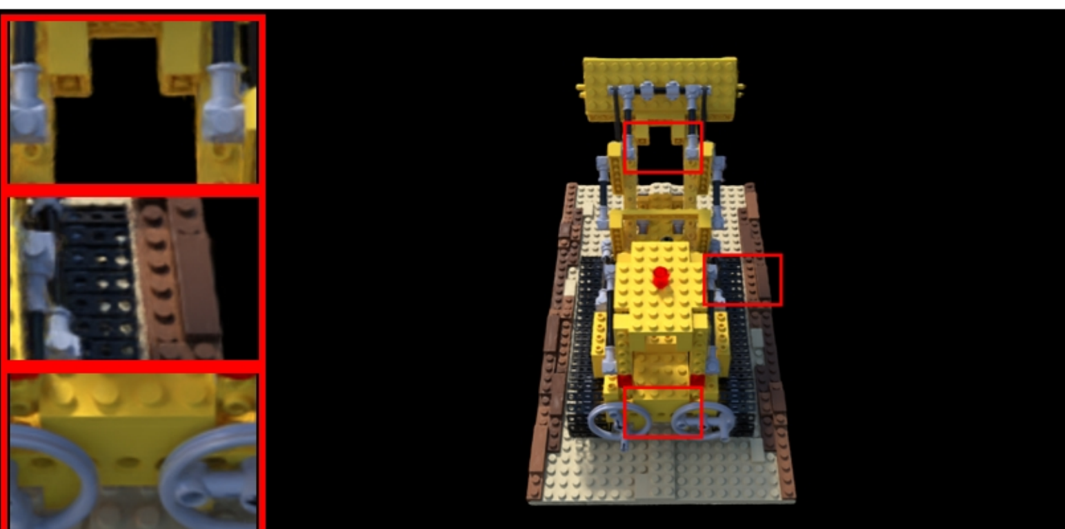
lego: VGGT | random | num_points=87000 PSNR: 20.62 | LPIPS: 0.0951 | SSIM: 0.7749
