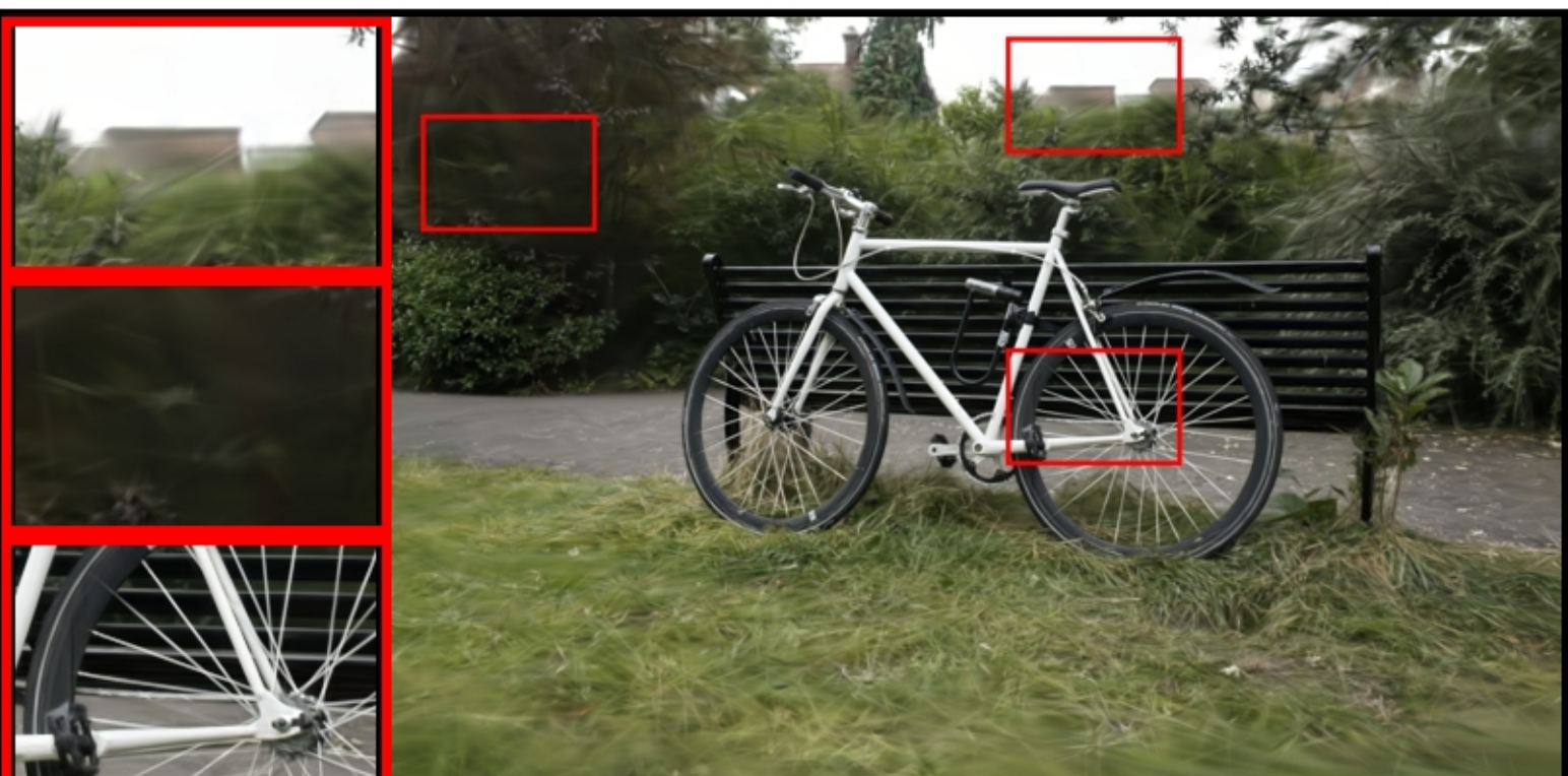
bicycle: COLMAP | | num_points=17352 PSNR: 21.33 | LPIPS: 0.3638 | SSIM: 0.4795
