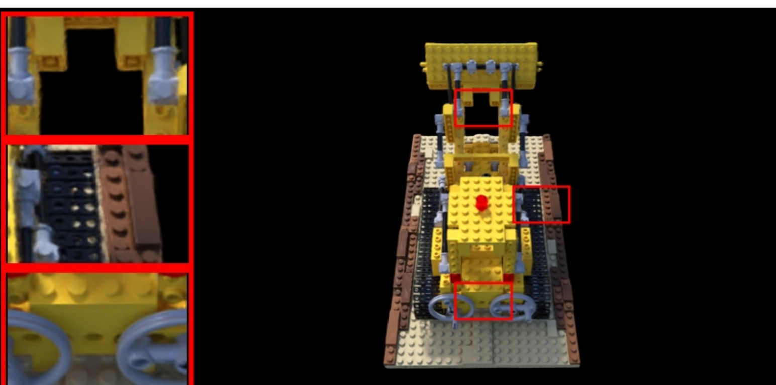
lego: VGGT | confidence | num_points=87000 PSNR: 20.61 | LPIPS: 0.0946 | SSIM: 0.7750
