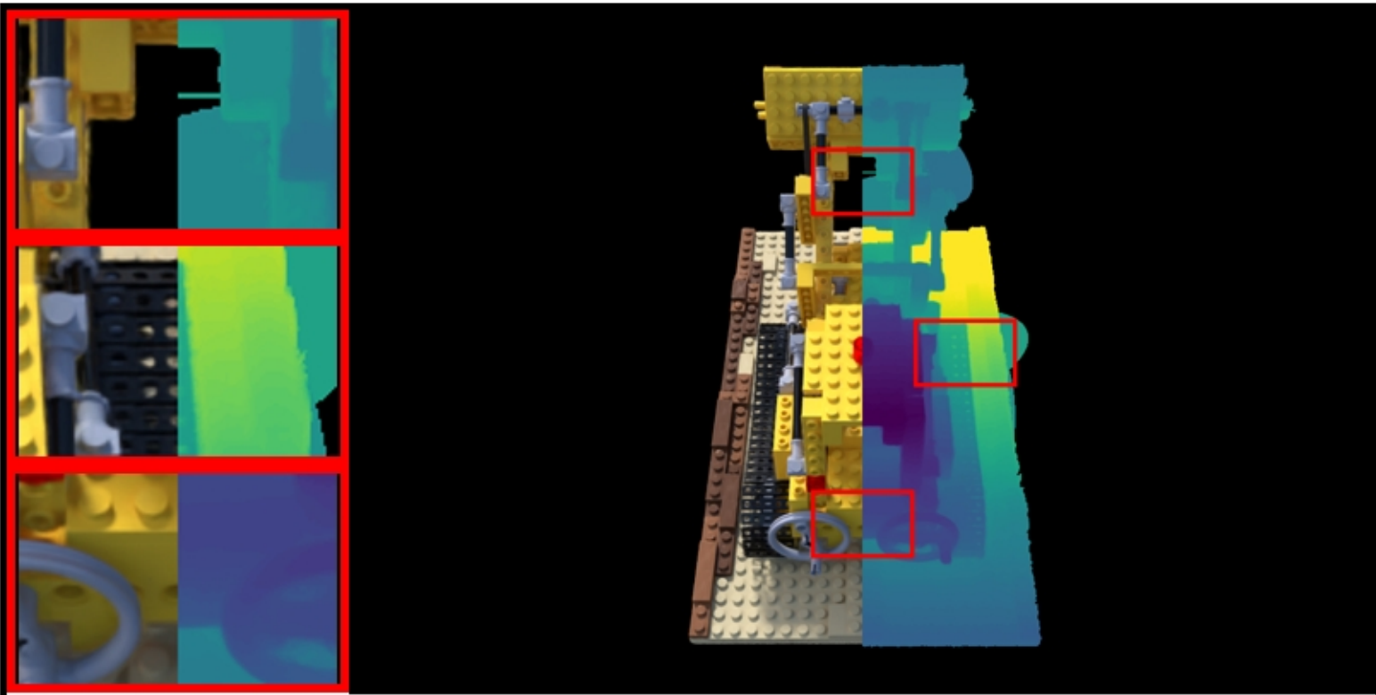
lego: VGGT | sigmoid PSNR: 21.97 | LPIPS: 0.0696 | SSIM: 0.8122
