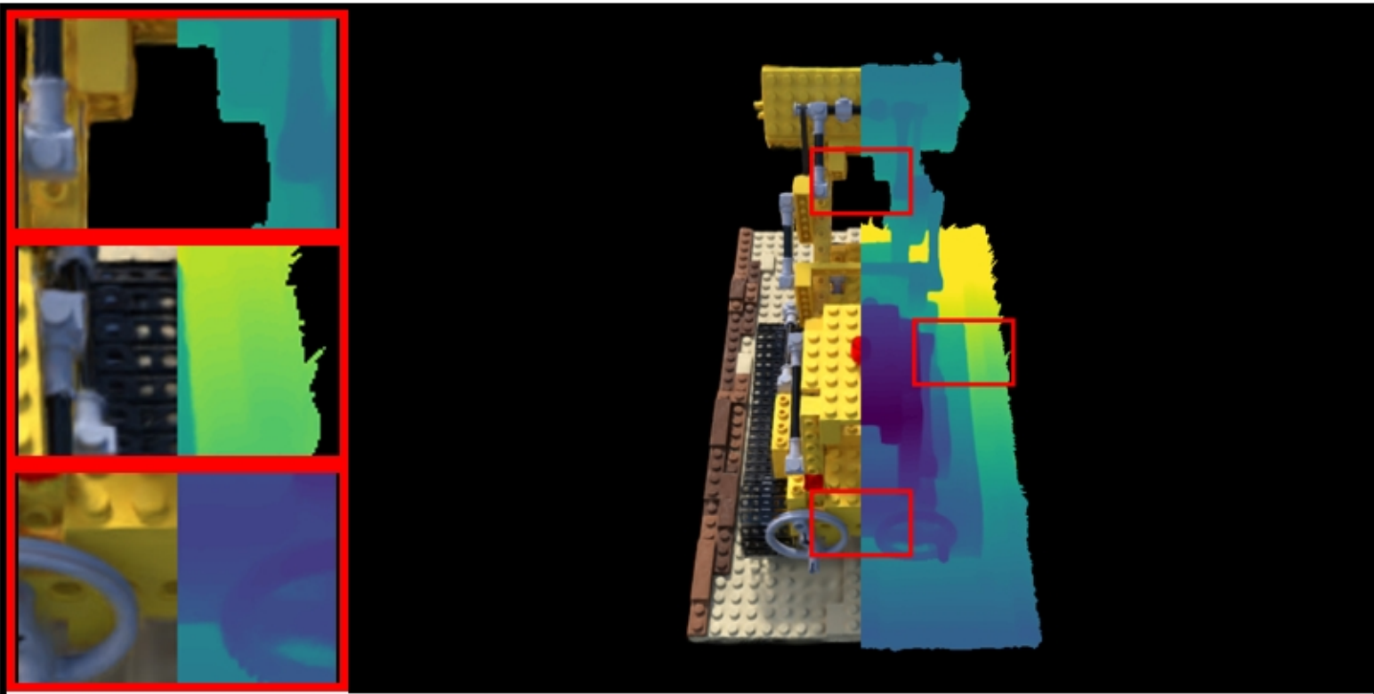
lego: VGGT | shifted PSNR: 23.51 | LPIPS: 0.0943 | SSIM: 0.8451
