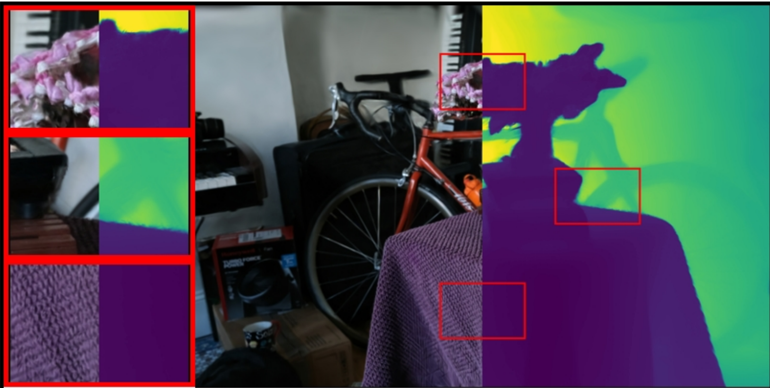
bonsai: VGGT | shifted PSNR: 17.55 | LPIPS: 0.3942 | SSIM: 0.5616
