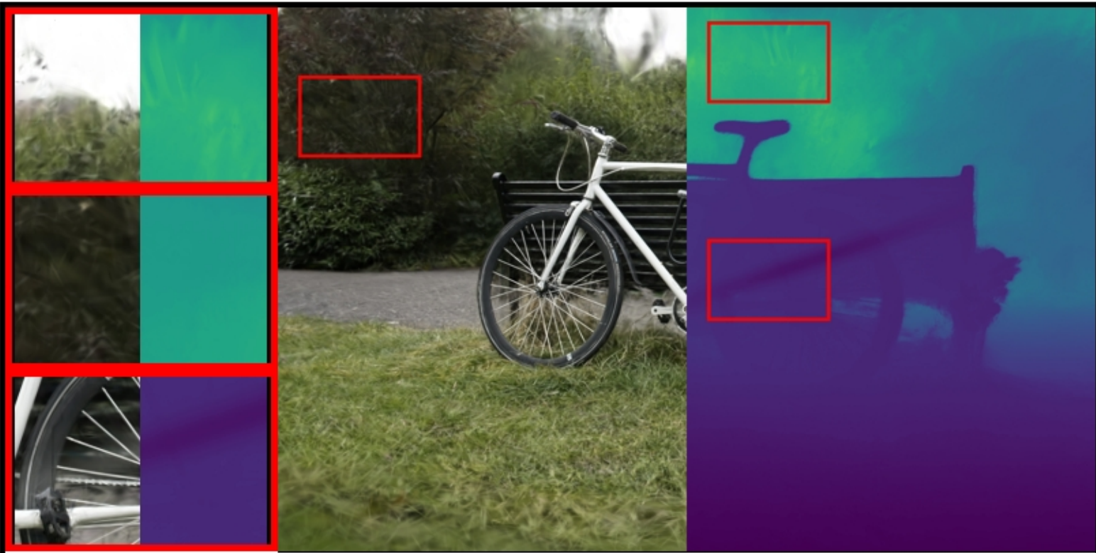
bicycle: VGGT | shifted PSNR: 18.09 | LPIPS: 0.3519 | SSIM: 0.2923
