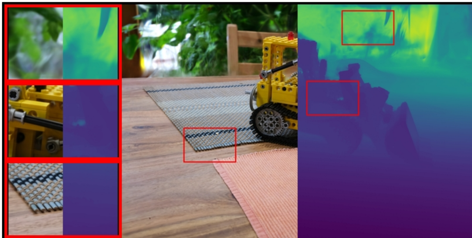
kitchen: VGGT | sigmoid PSNR: 19.09 | LPIPS: 0.2111 | SSIM: 0.4037
