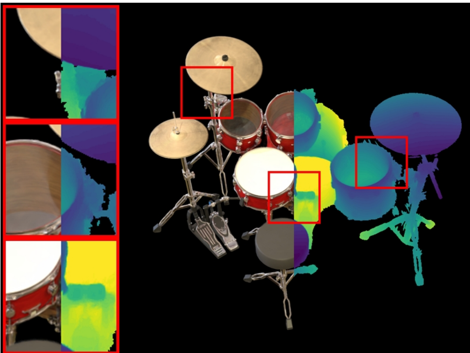
drums: VGGT | sigmoid PSNR: 20.87 | LPIPS: 0.0878 | SSIM: 0.8694
