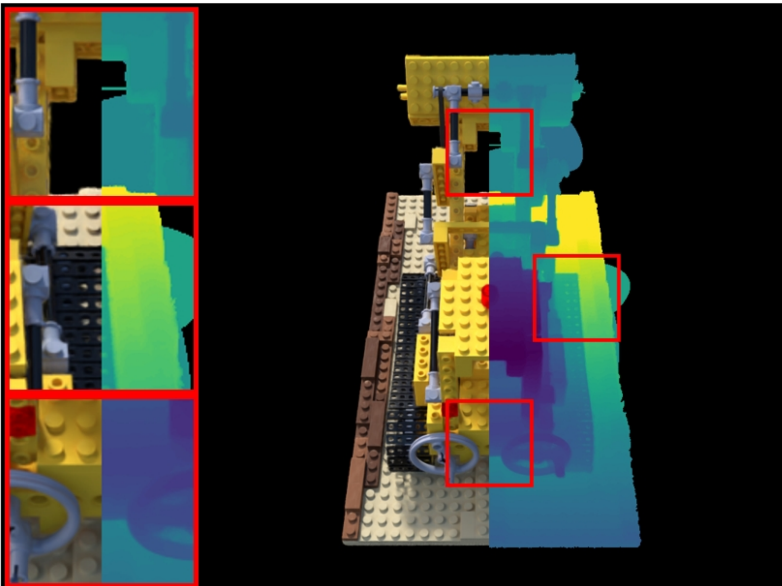
lego: VGGT | sigmoid PSNR: 21.97 | LPIPS: 0.0696 | SSIM: 0.8122
