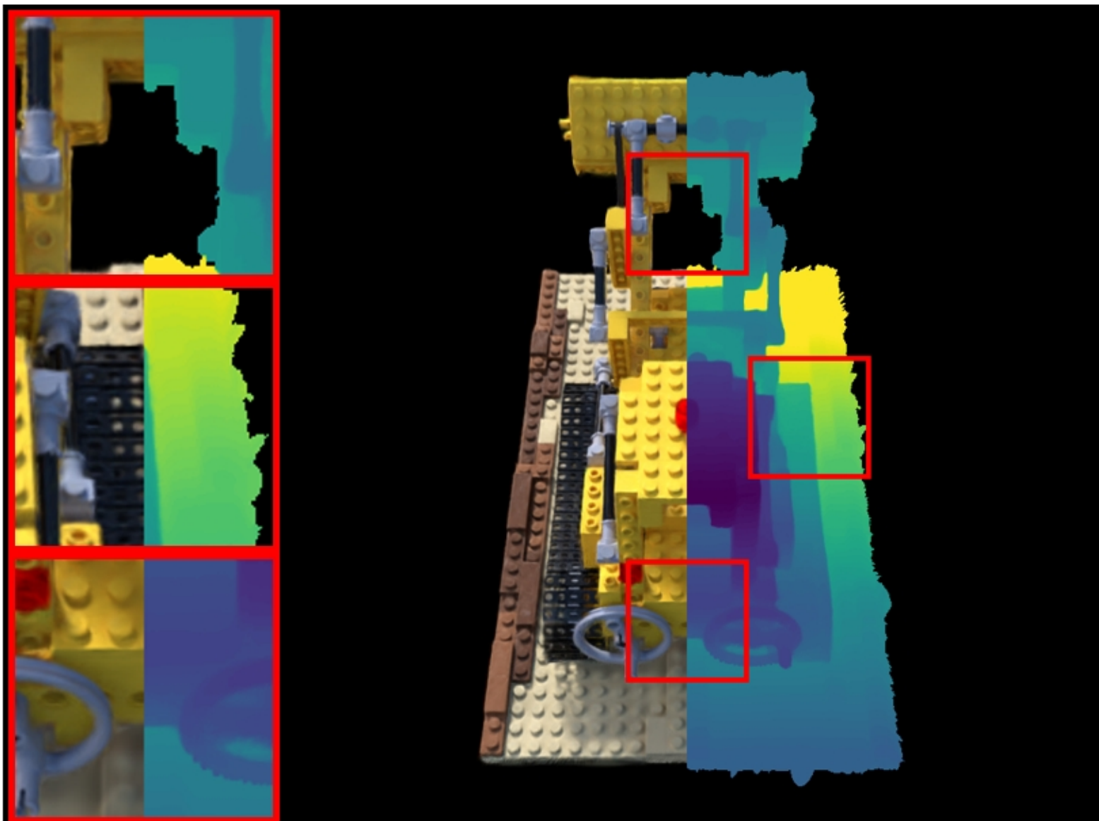
lego: VGGT | standard PSNR: 23.51 | LPIPS: 0.0945 | SSIM: 0.8450
