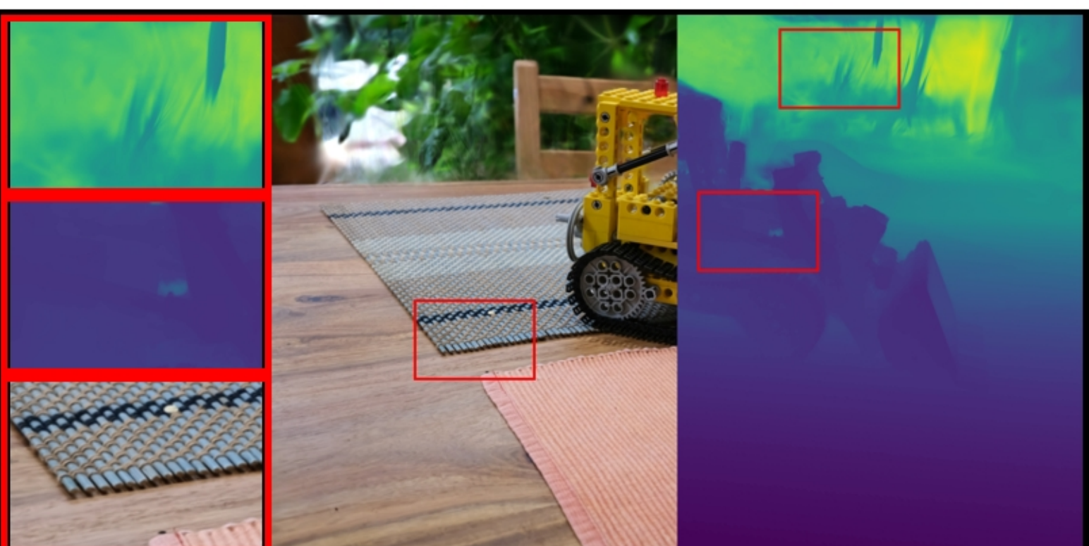
kitchen: VGGT | full PSNR: 19.04 | LPIPS: 0.2102 | SSIM: 0.4003
