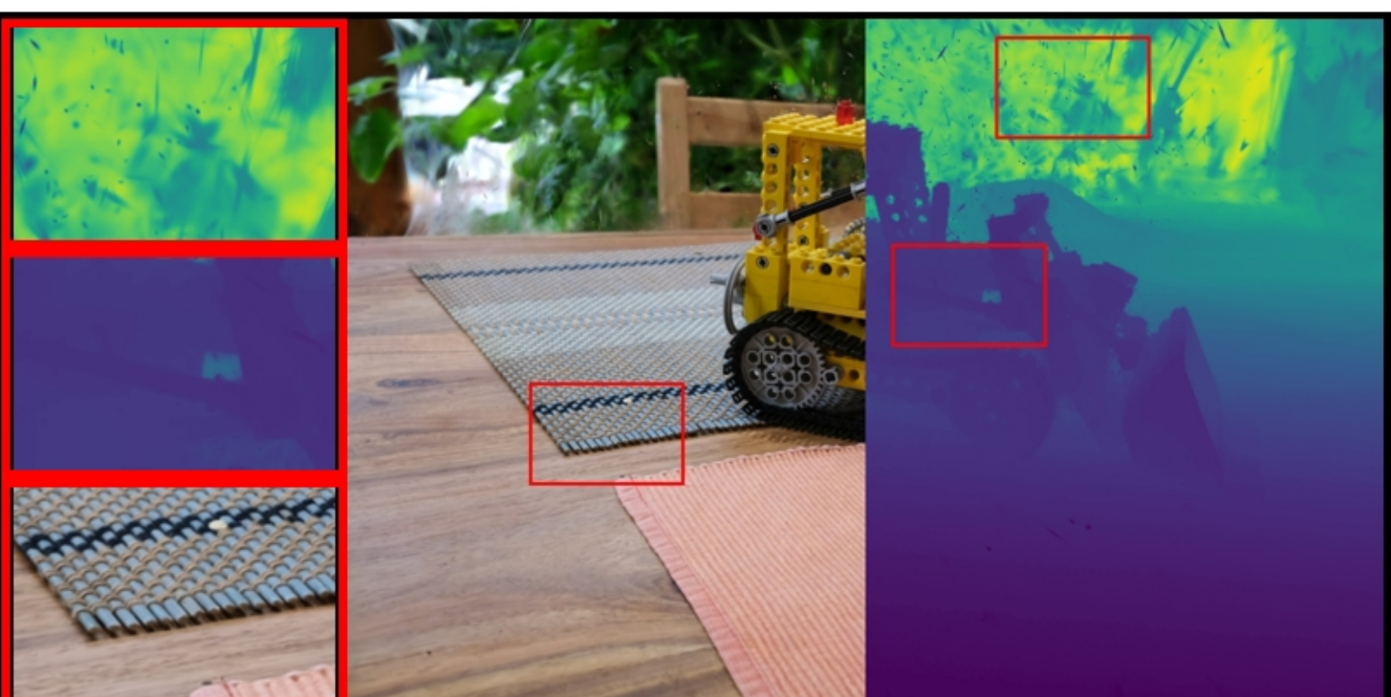
kitchen: VGGT | points PSNR: 19.31 | LPIPS: 0.2160 | SSIM: 0.4216
