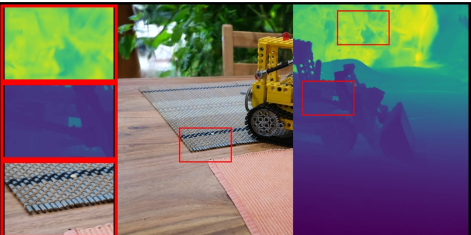
kitchen: VGGT | PSNR: 20.02 | LPIPS: 0.1764 | SSIM: 0.4138
