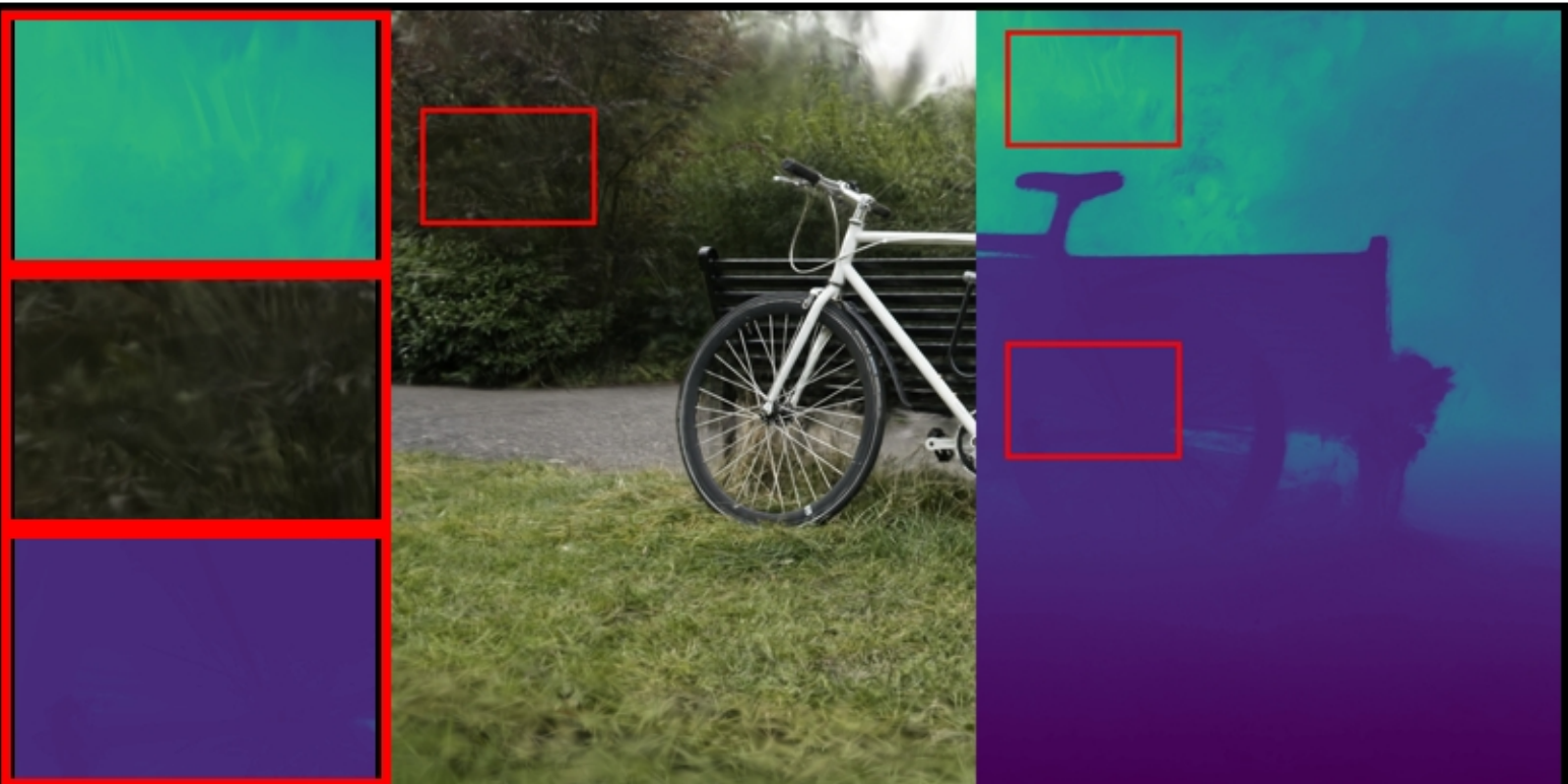
bicycle: VGGT | full PSNR: 18.11 | LPIPS: 0.3513 | SSIM: 0.2933
