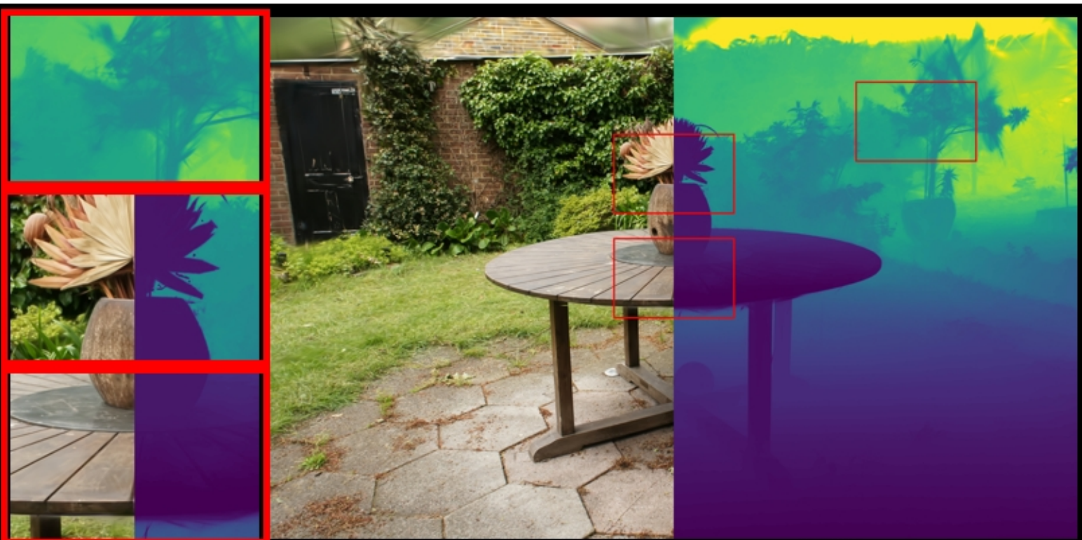
garden: COLMAP | points PSNR: 21.96 | LPIPS: 0.2716 | SSIM: 0.4987
