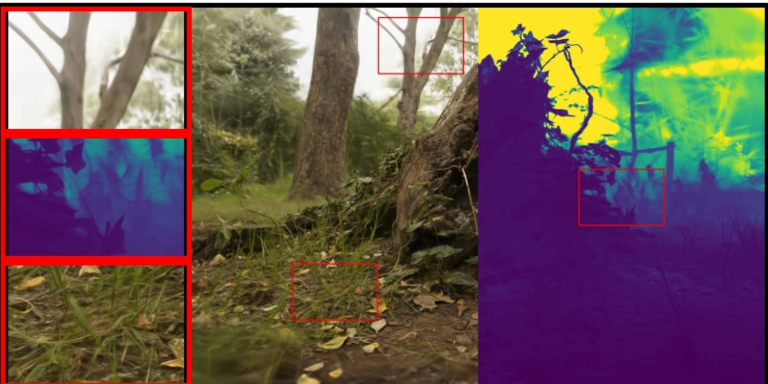
stump: COLMAP | PSNR: 24.83 | LPIPS: 0.3404 | SSIM: 0.6965
