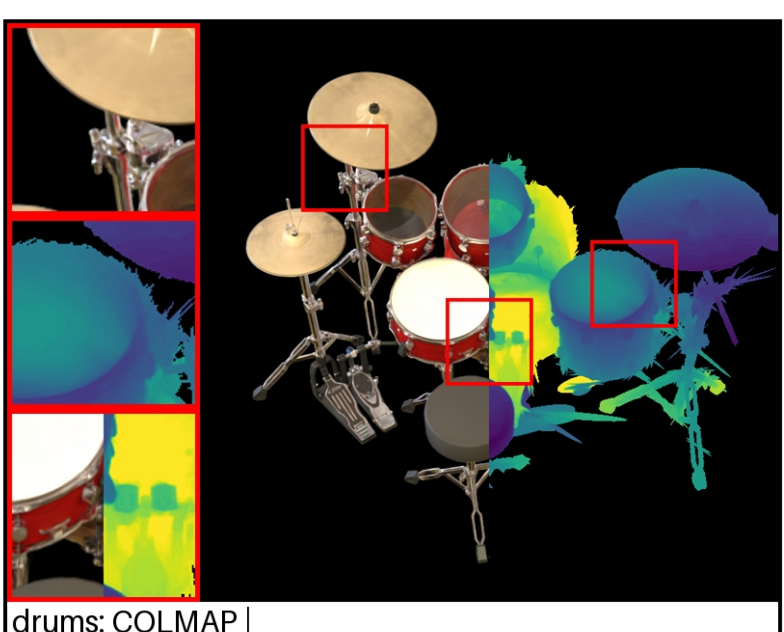
drums: COLMAP | PSNR: 22.80 | LPIPS: 0.0892 | SSIM: 0.9061
