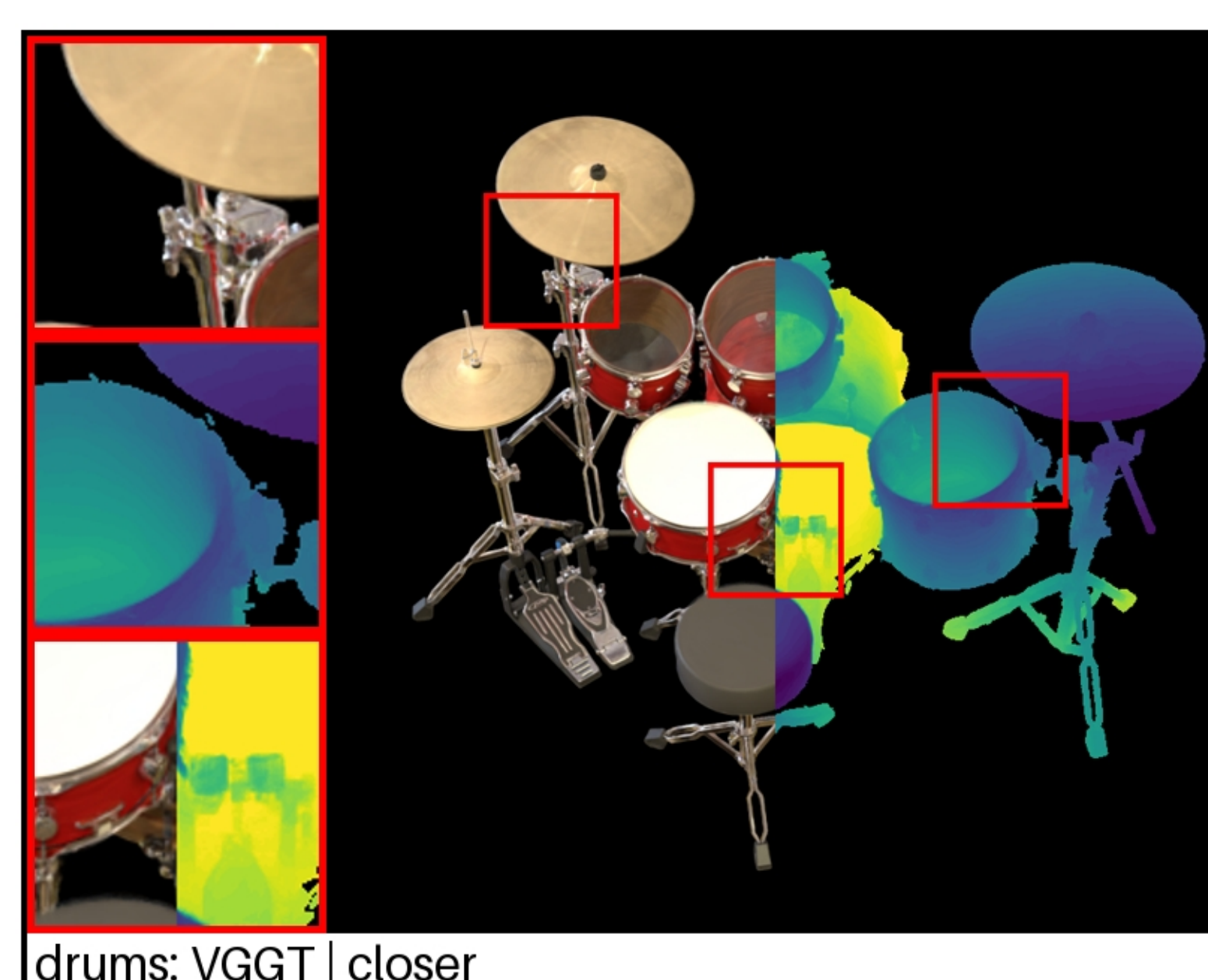
drums: VGGT | closer PSNR: 20.03 | LPIPS: 0.0915 | SSIM: 0.8510
