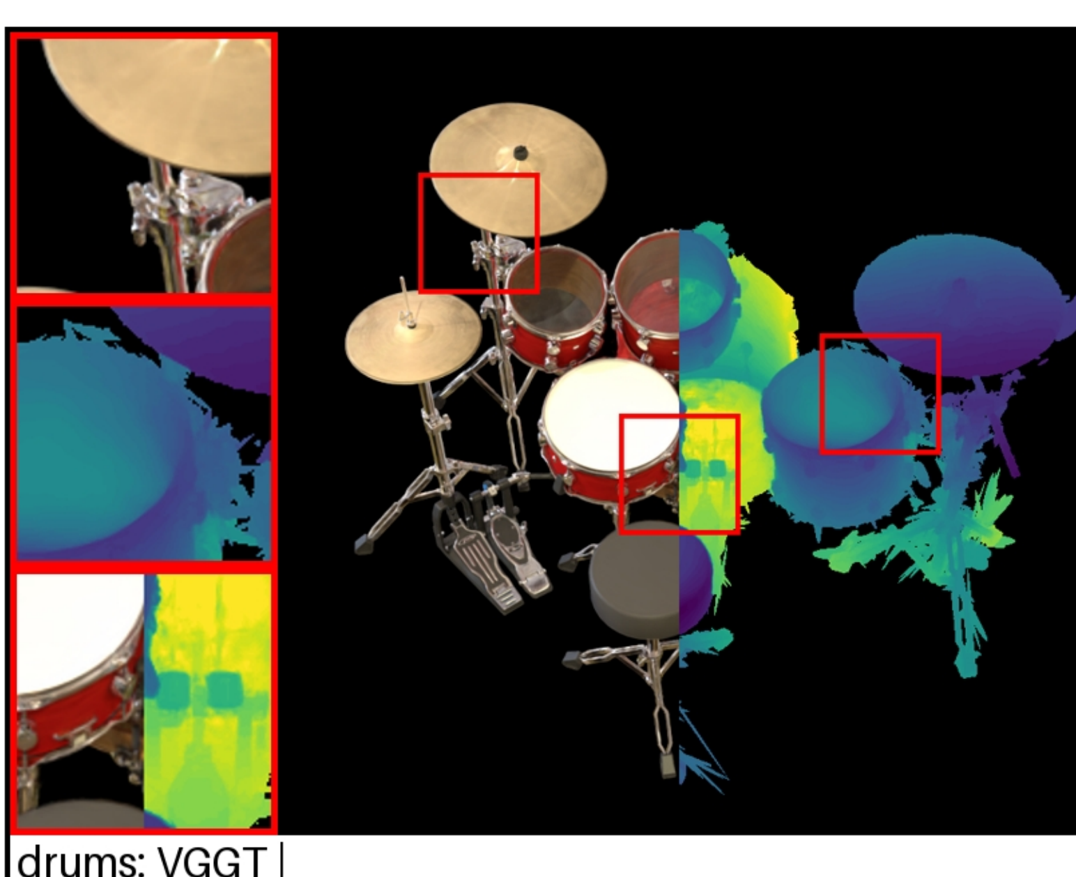
drums: VGGT | PSNR: 20.90 | LPIPS: 0.0848 | SSIM: 0.8690
