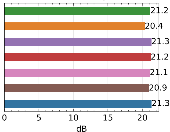
PSNR ↑ - bicycle
