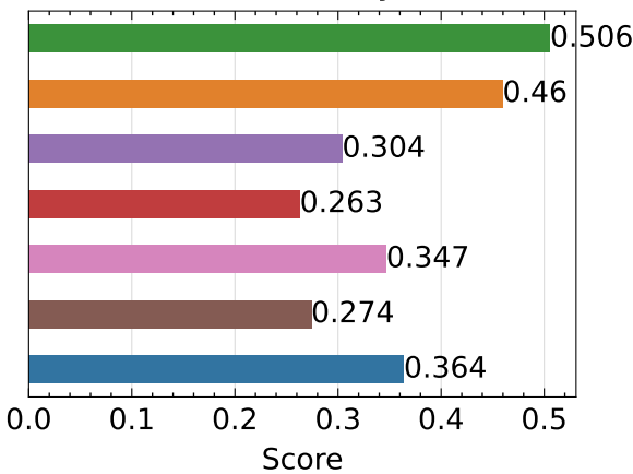
LPIPS ↓ - bicycle
