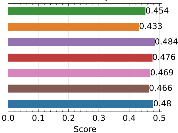
SSIM ↑ - bicycle
