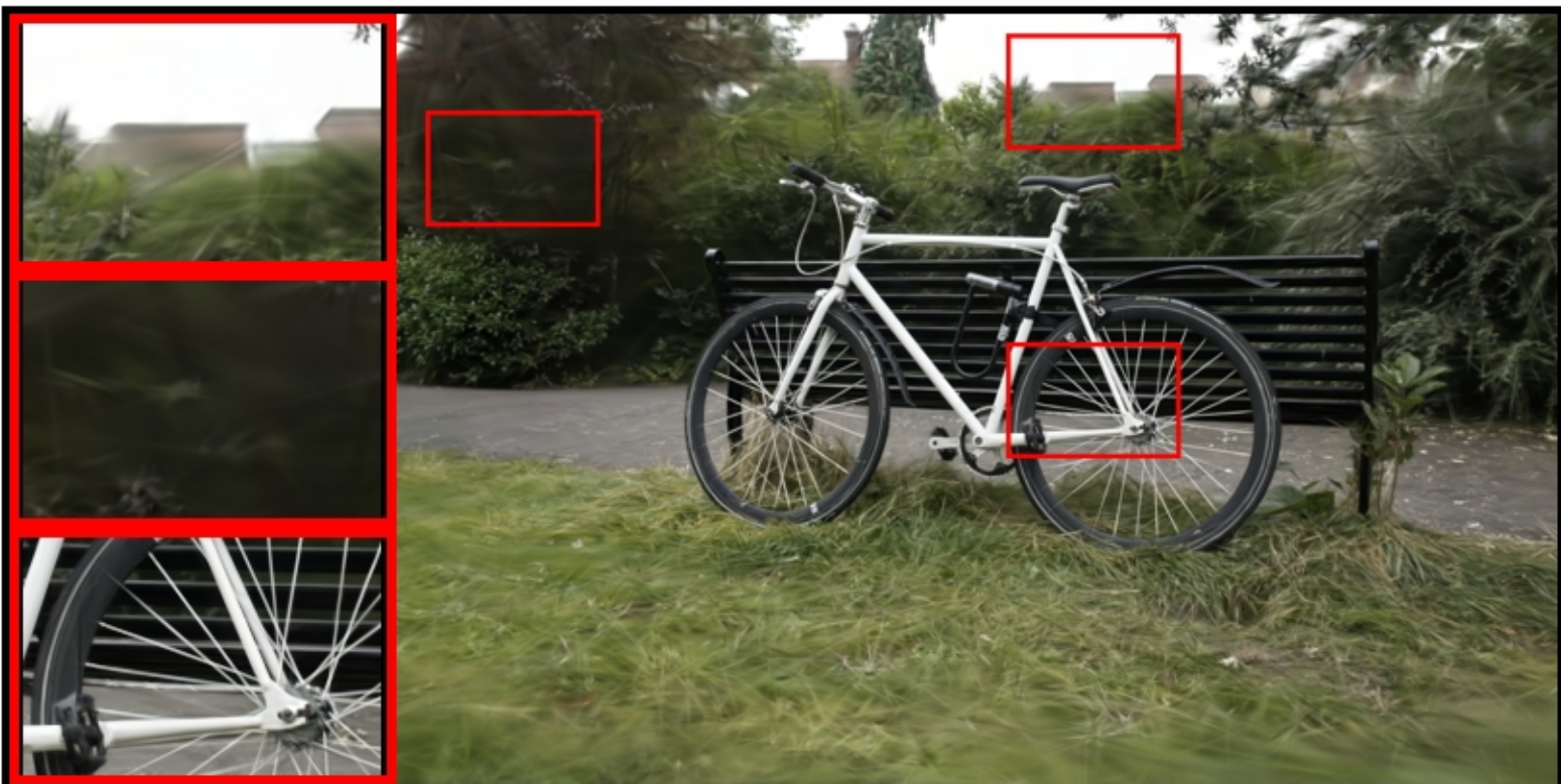
bicycle: COLMAP | | | 17352 PSNR: 21.33 | LPIPS: 0.3638 | SSIM: 0.4795
