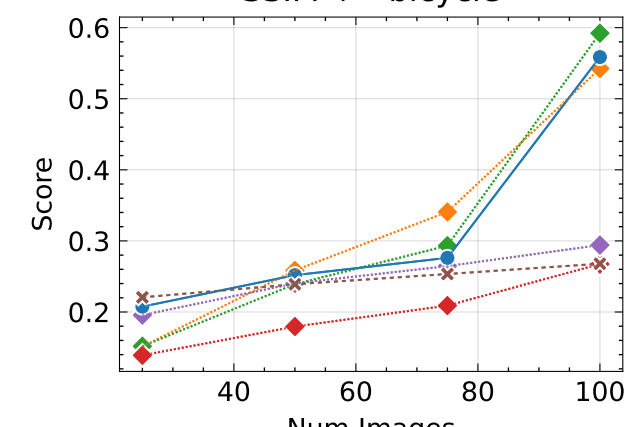
SSIM ↑ - bicycle
