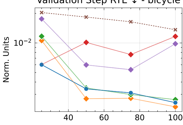
Validation Step RTE ↓ - bicycle
