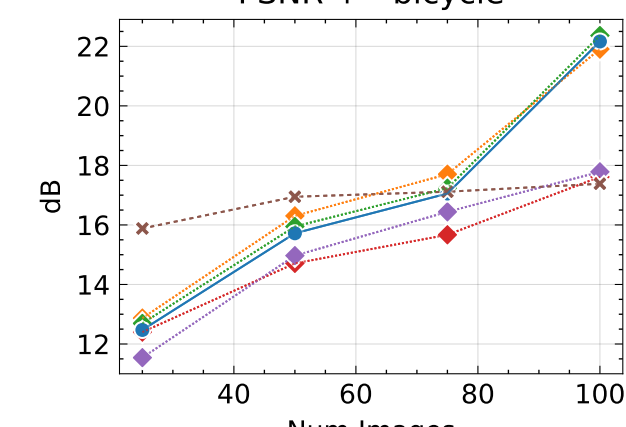
PSNR ↑ - bicycle
