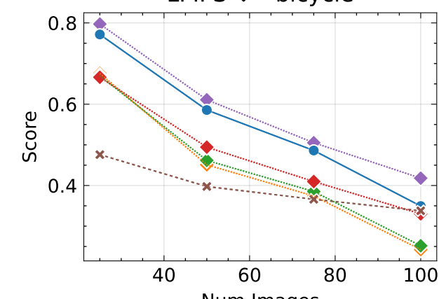
LPIPS ↓ - bicycle
