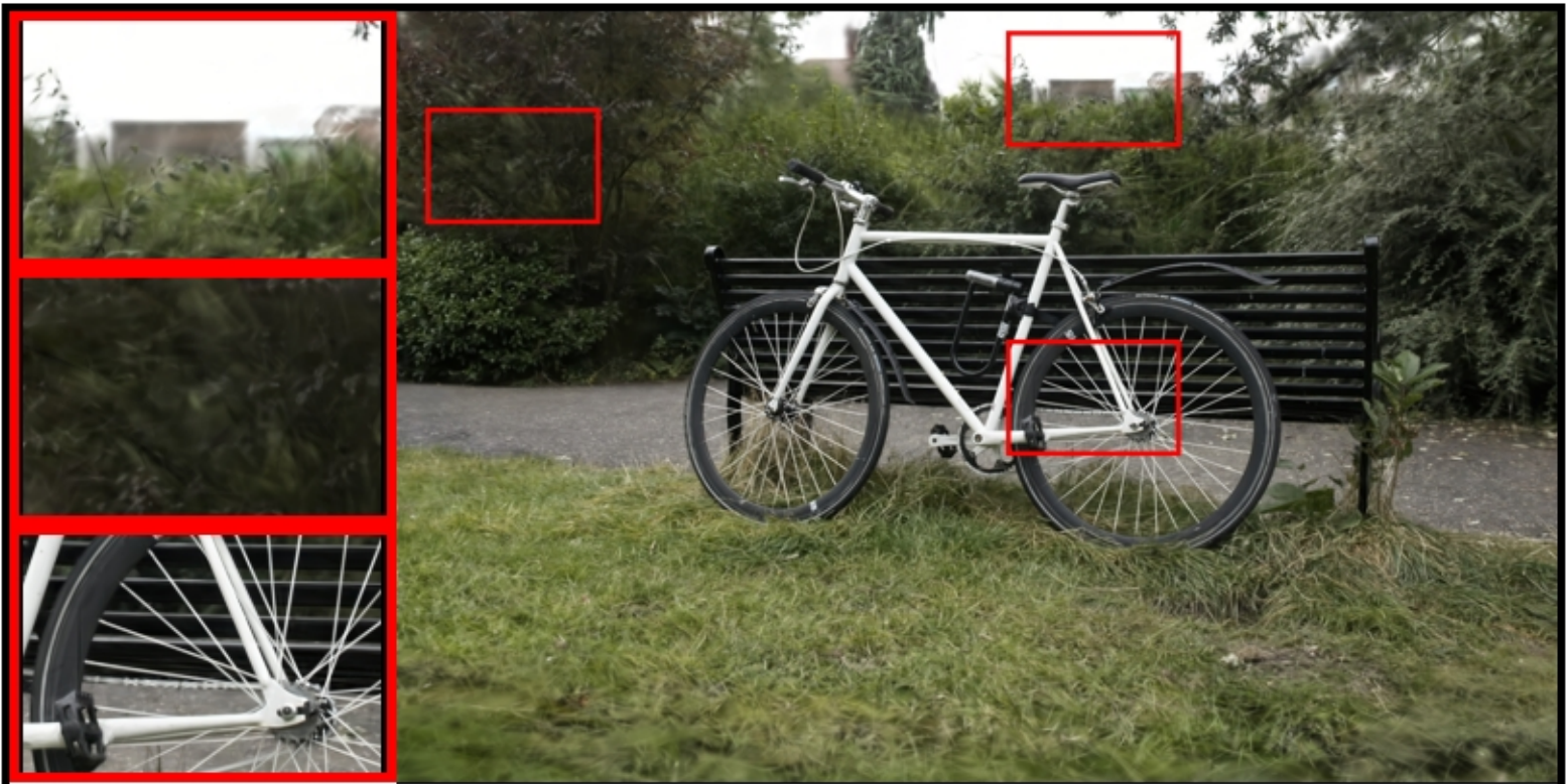
bicycle: Combined | COLMAP Cams | Both Pcds | num_in PSNR: 21.91 | LPIPS: 0.2423 | SSIM: 0.5425
