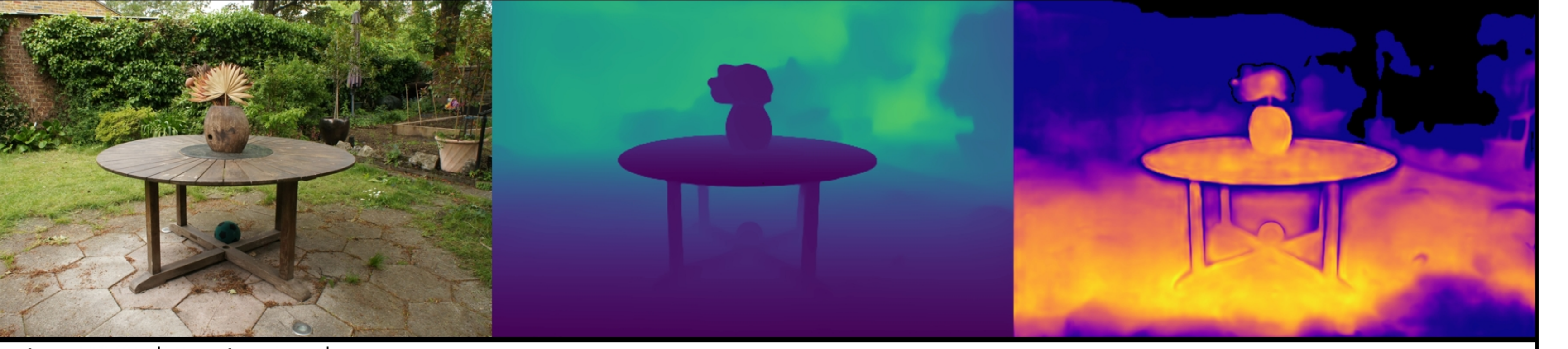
garden: VGGT | Random Init | Use BA Original | Depth (max=2.46) | Confidence (max=6.23)
