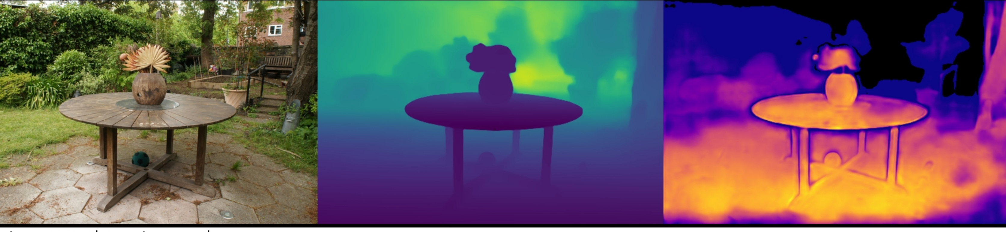
garden: VGGT | Random Init | Use BA Original | Depth (max=2.65) | Confidence (max=6.53)
