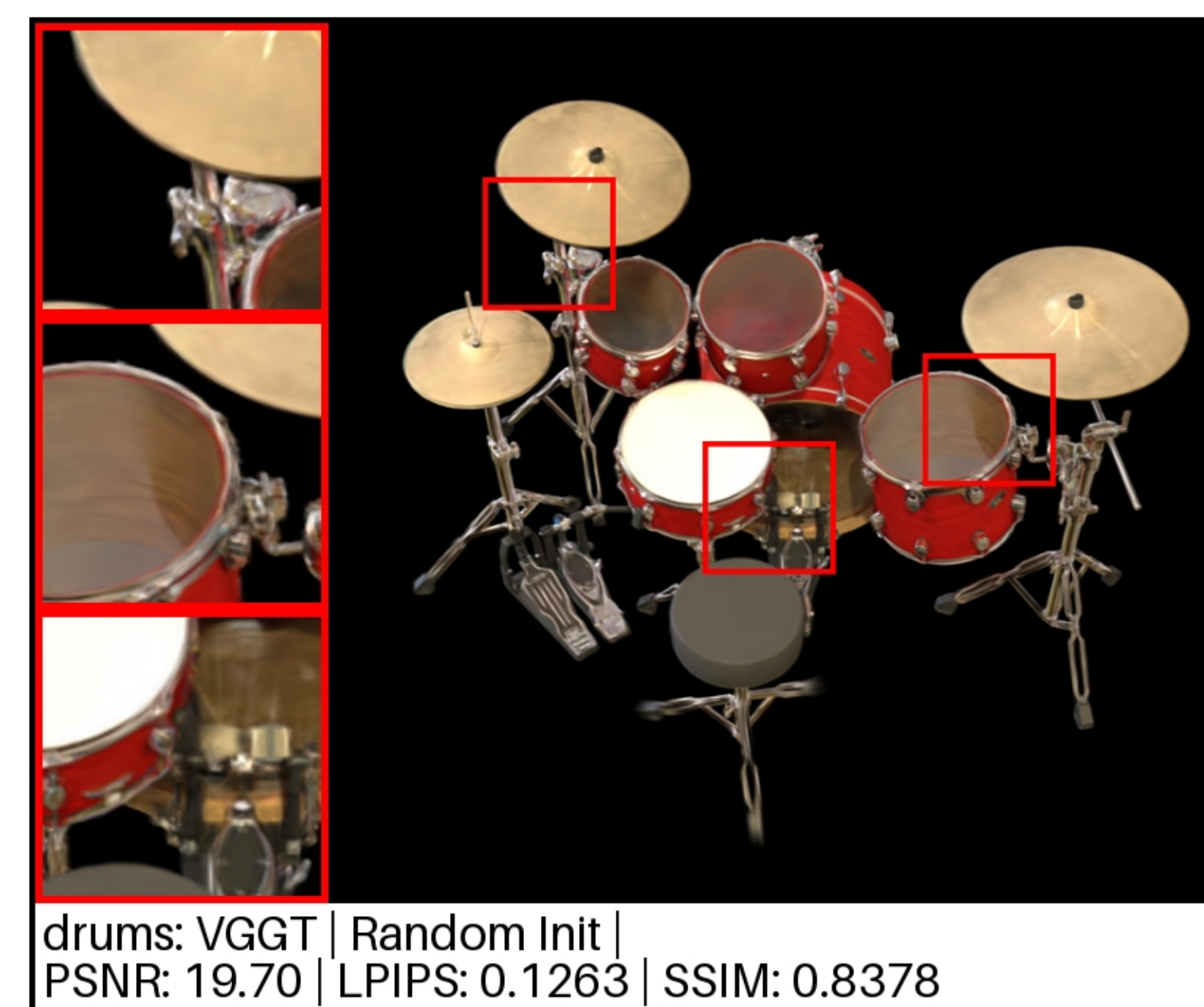
drums: VGGT | Random Init | PSNR: 19.70 | LPIPS: 0.1263 | SSIM: 0.8378
