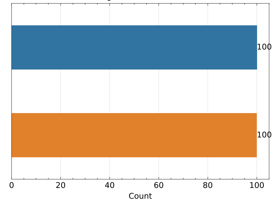
Aligned Cameras ↑
