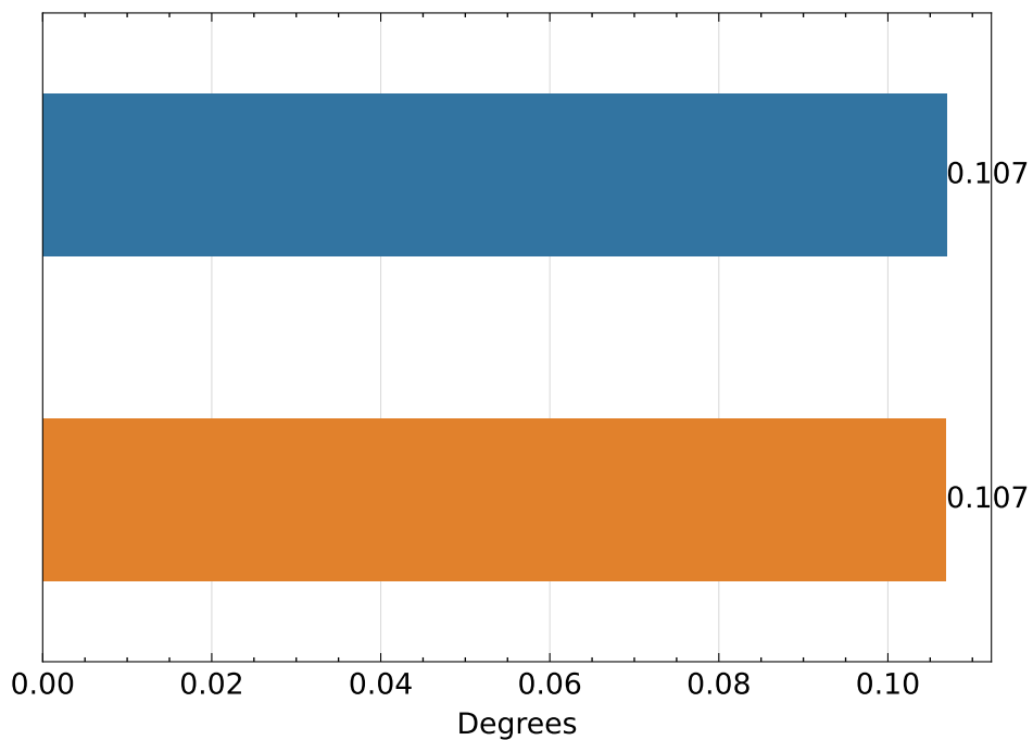
Aligned Cameras ↑
