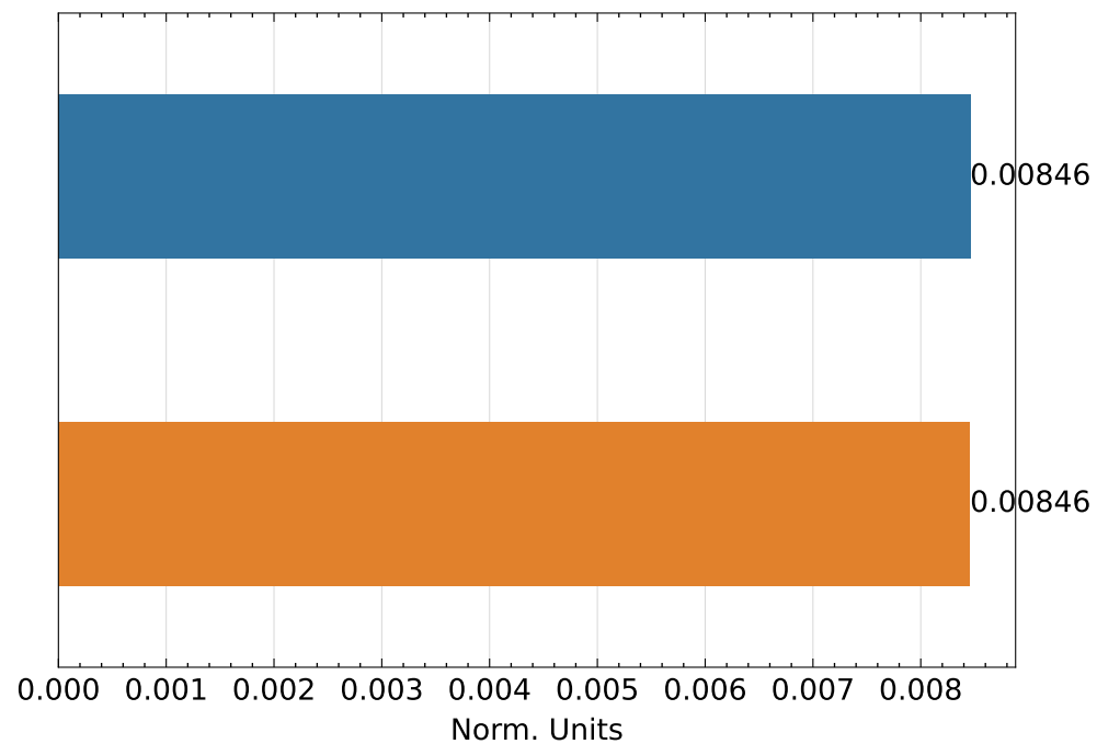
Composite Quality ↑
