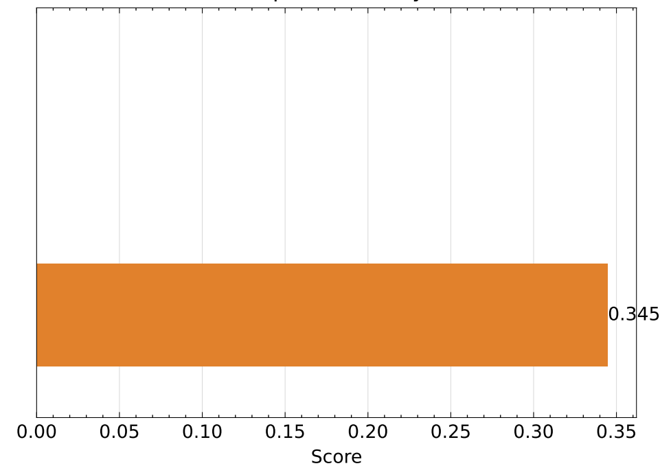
Composite Quality ↑
