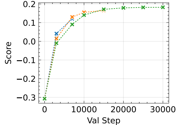
Composite Quality ↑
