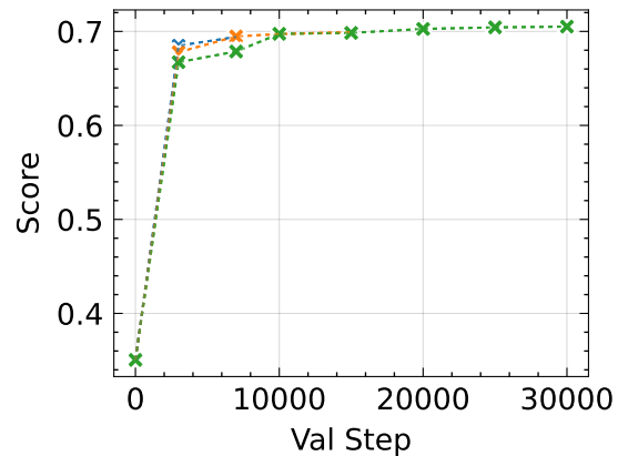
Composite Quality ↑
