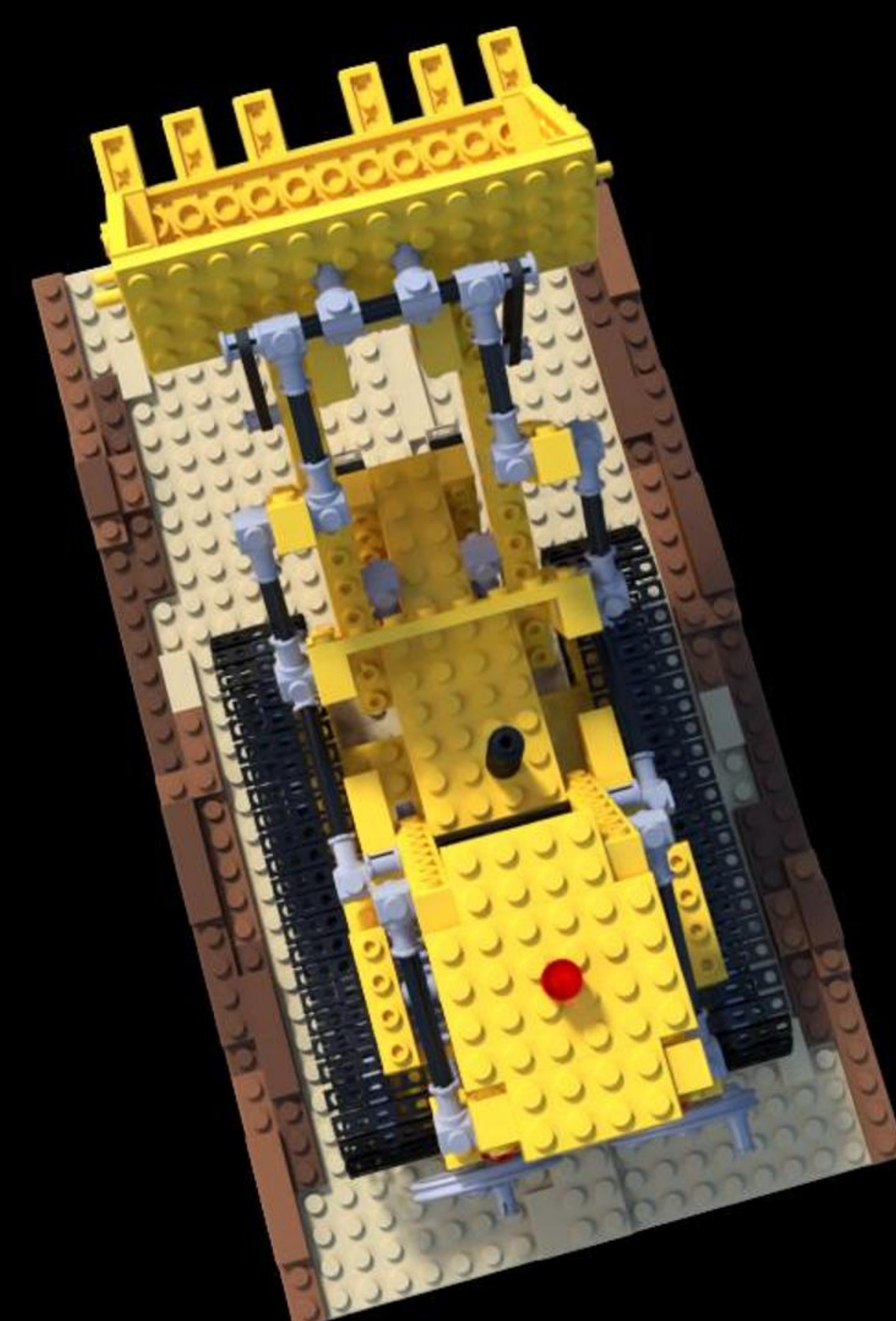
Config: COLMAP | GT Extrinsic | GT Intrinsic | PSNR: 34.62 | LPIPS: 0.0241 | SSIM: 0.9851
