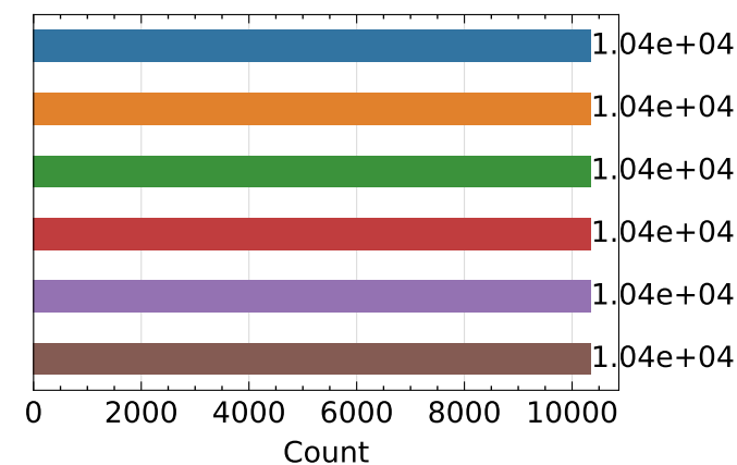
Initial Points
