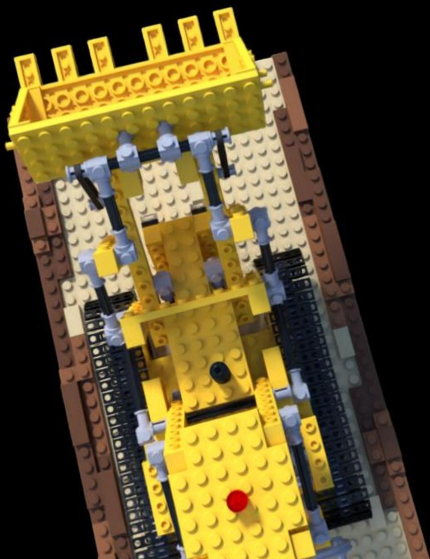
Config: Combined | | VGGTpcd | 10350 PSNR: 9.42 | LPIPS: 0.5635 | SSIM: 0.5178
