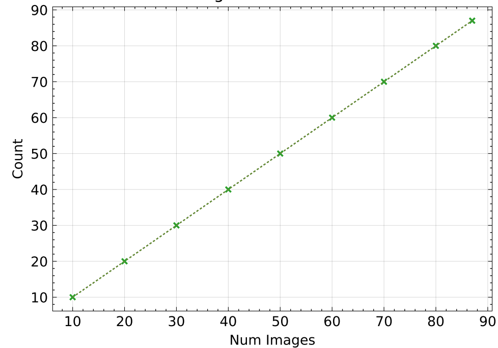
Aligned Cameras ↑
