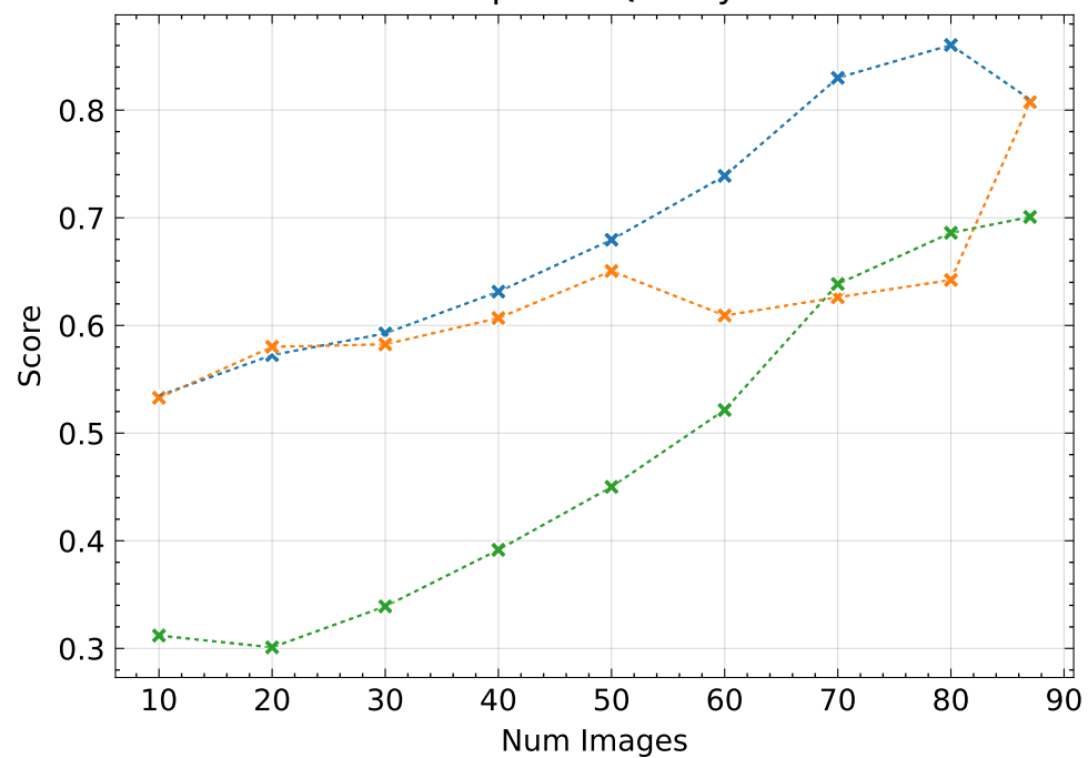
Composite Quality ↑
