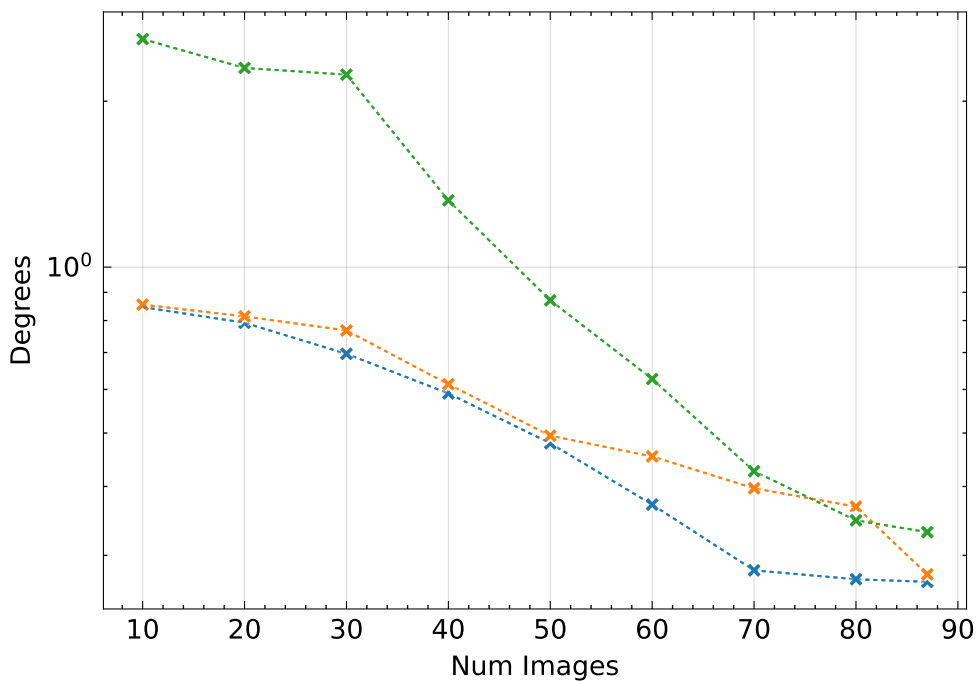
Aligned Cameras ↑
