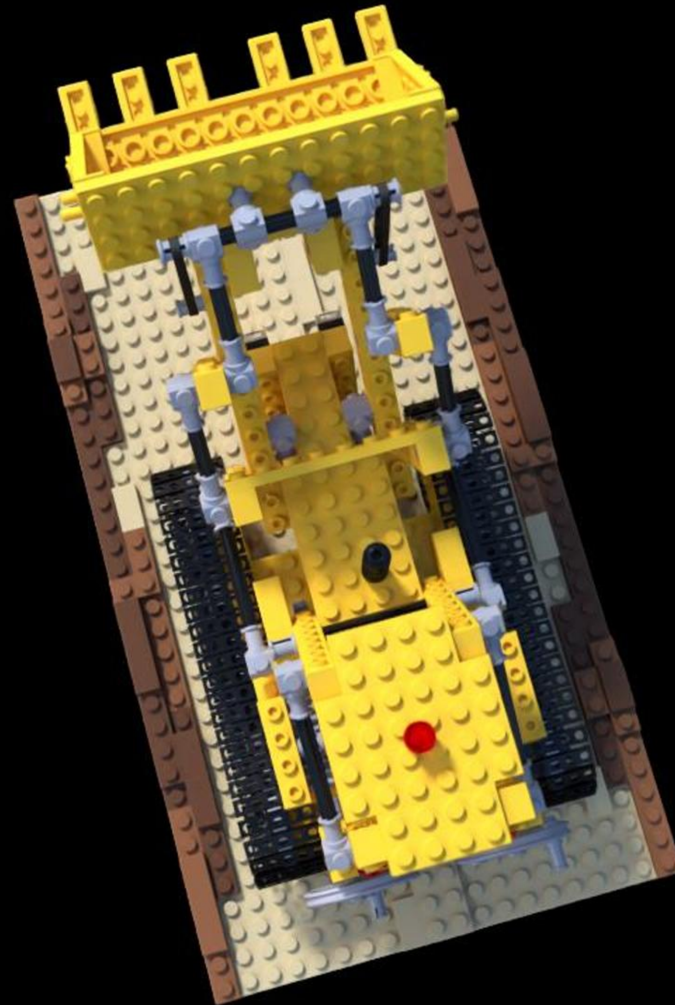
Config: VGGT | | num_images=87 PSNR: 21.11 | LPIPS: 0.0583 | SSIM: 0.8017
