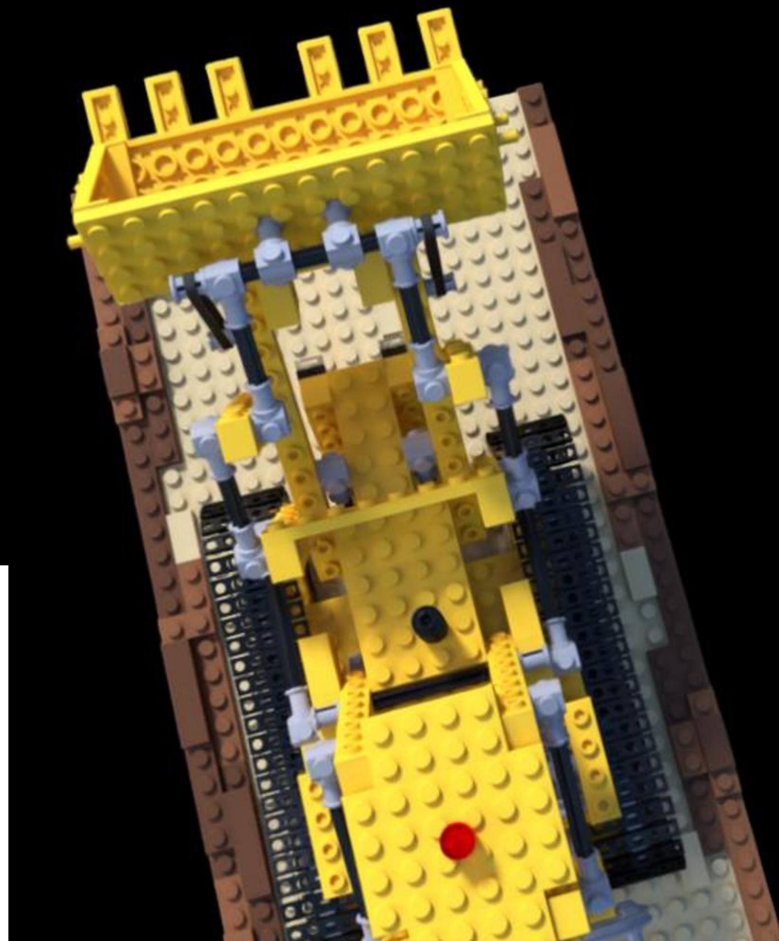
Config: COLMAP | | num_points=10350 PSNR: 9.41 | LPIPS: 0.5630 | SSIM: 0.5177
