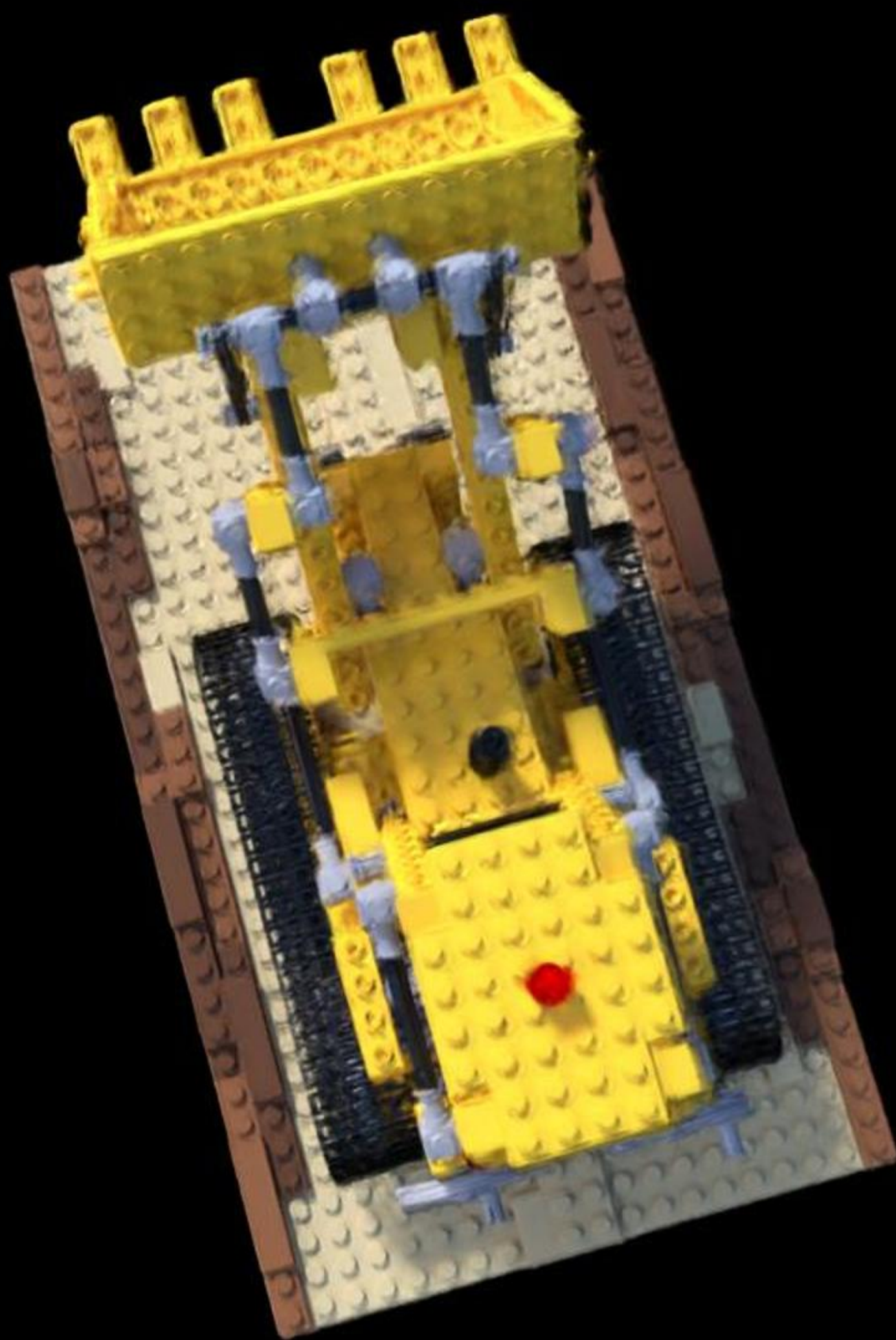
Config: VGGT | | num_images=80 PSNR: 18.45 | LPIPS: 0.1210 | SSIM: 0.7316
