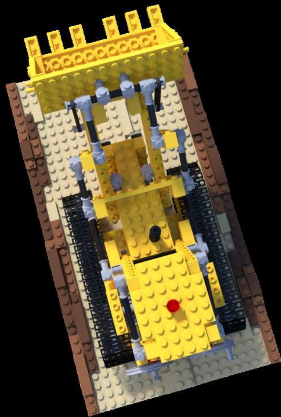
Ground Truth
