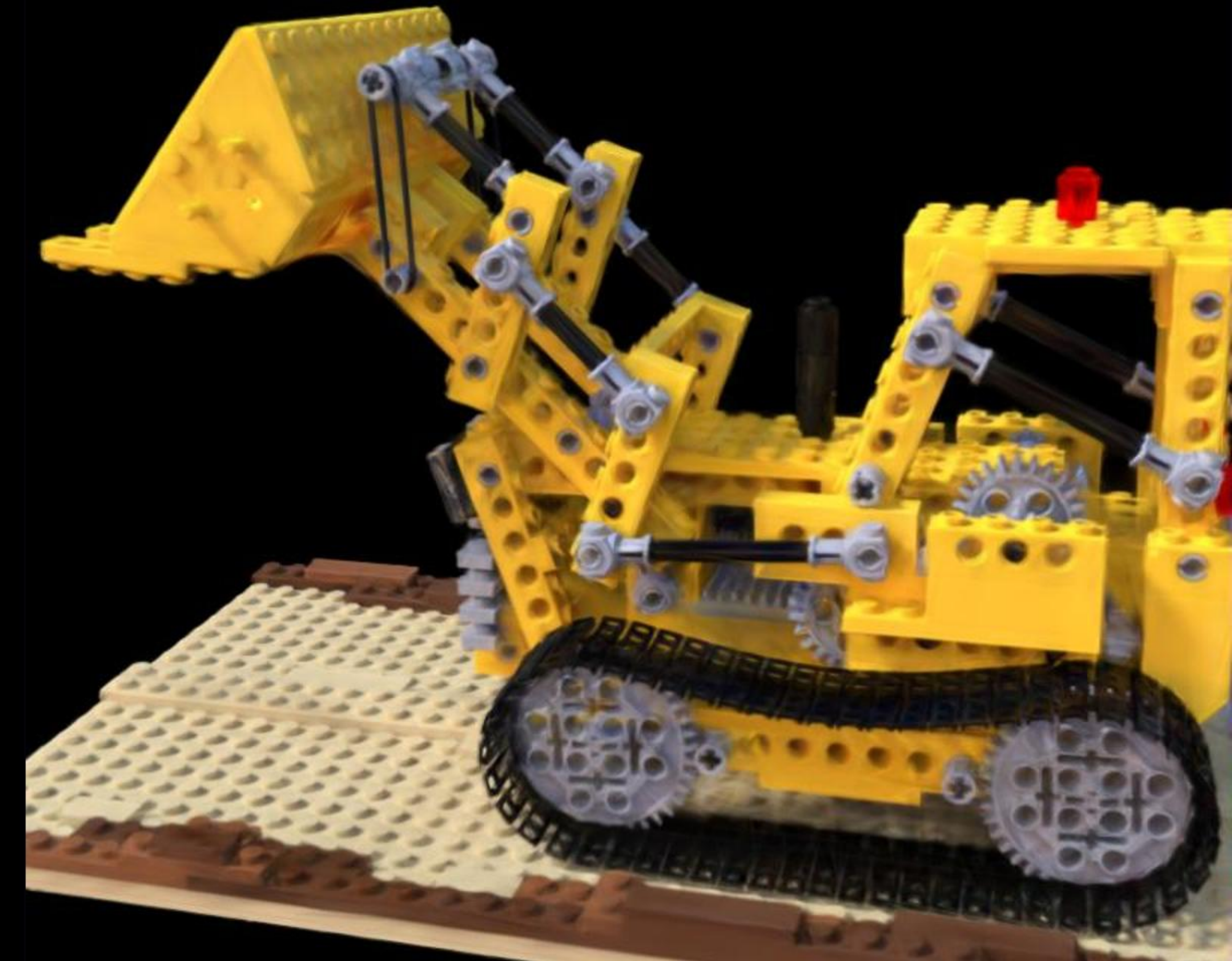
Config: COLMAP | | default PSNR: 8.28 | LPIPS: 0.6681 | SSIM: 0.3801
