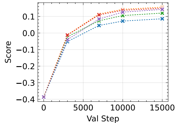
Composite Quality ↑
