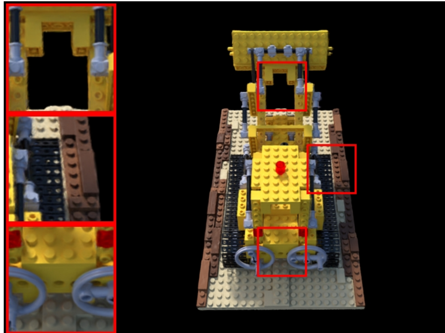
lego: VGGT | num_images=87 PSNR: 20.57 | LPIPS: 0.0950 | SSIM: 0.7737
