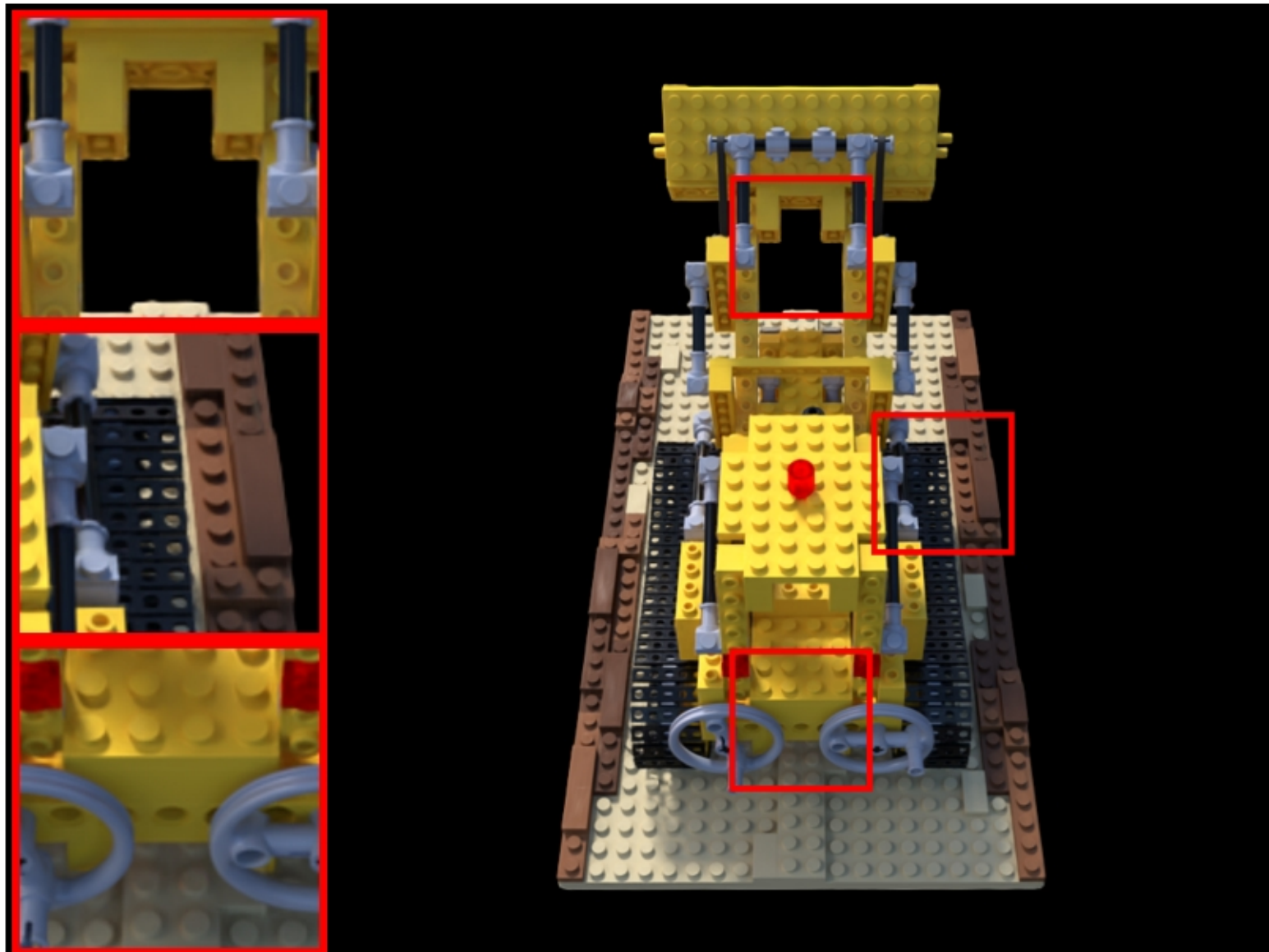
lego: COLMAP | num_images=87 PSNR: 22.79 | LPIPS: 0.0657 | SSIM: 0.8508
