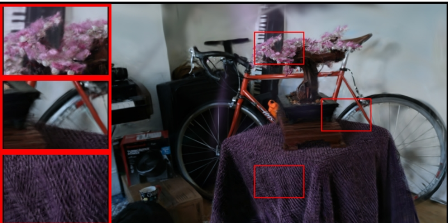
bonsai: VGGT | imagefps | num_points=100000 PSNR: 18.60 | LPIPS: 0.3913 | SSIM: 0.5943
