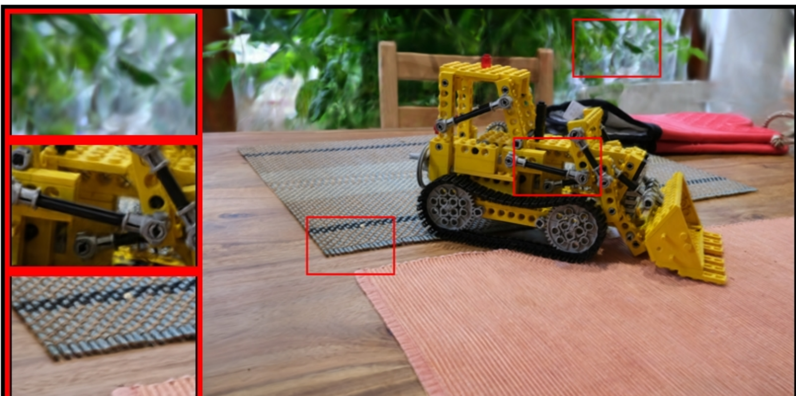
kitchen: VGGT | random | num_points=100000 PSNR: 20.49 | LPIPS: 0.2296 | SSIM: 0.4849
