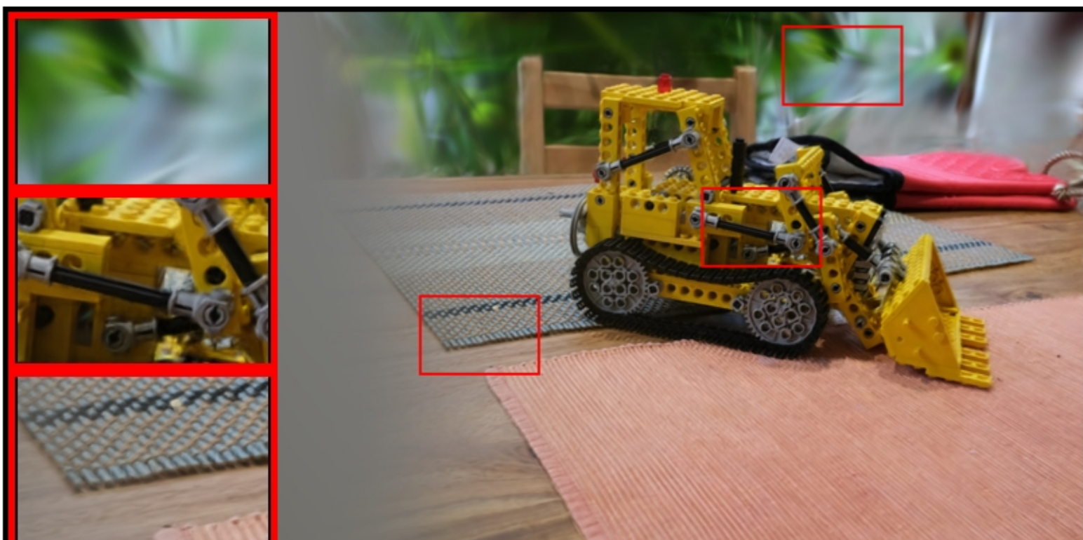
kitchen: VGGT | voxels | num_points=100000 PSNR: 20.26 | LPIPS: 0.2519 | SSIM: 0.4869
