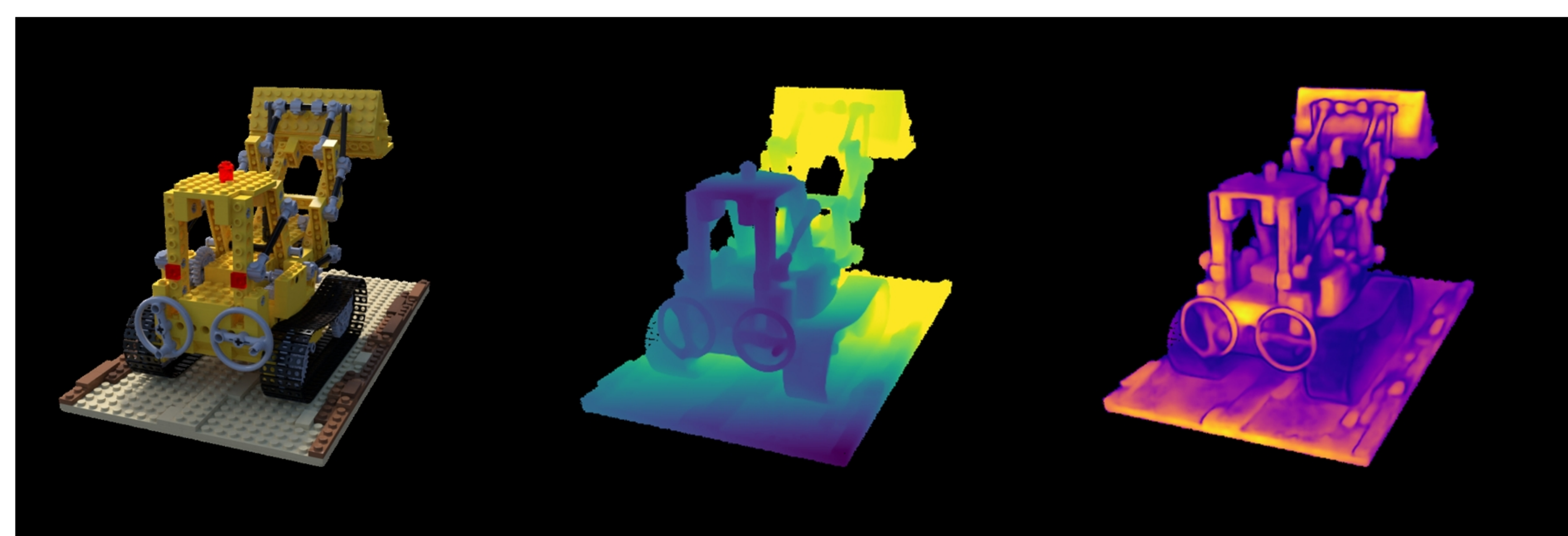
lego: VGGT | voxels | num_points=87000 Original | Depth (max=1.28) | Confidence (max=155.74)
