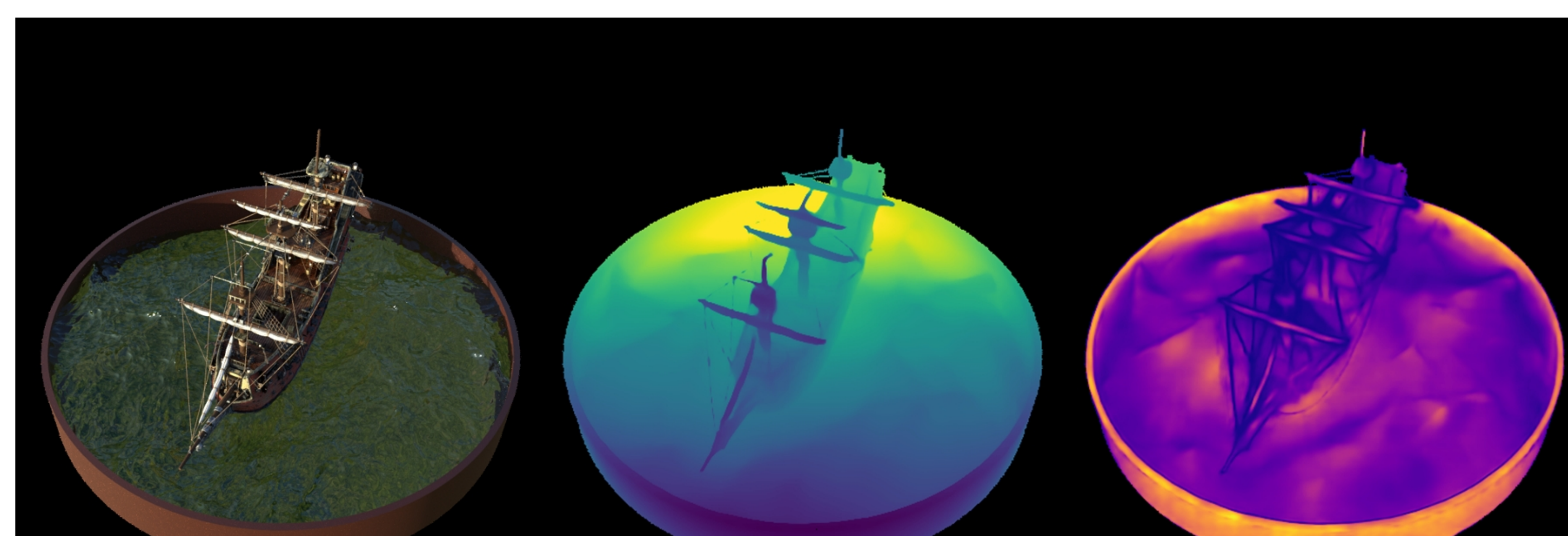
ship: VGGT | voxels | num_points=87000 Original | Depth (max=1.23) | Confidence (max=146.85)
