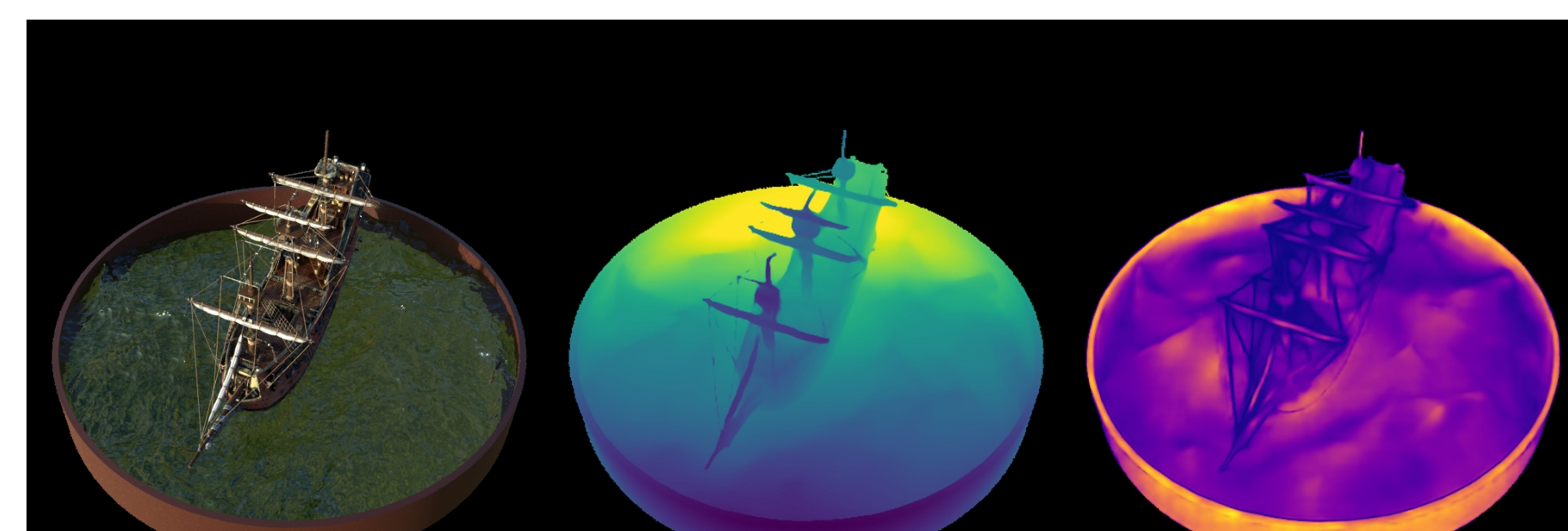
ship: VGGT | imagefps | num_points=87000 Original | Depth (max=1.23) | Confidence (max=146.85)
