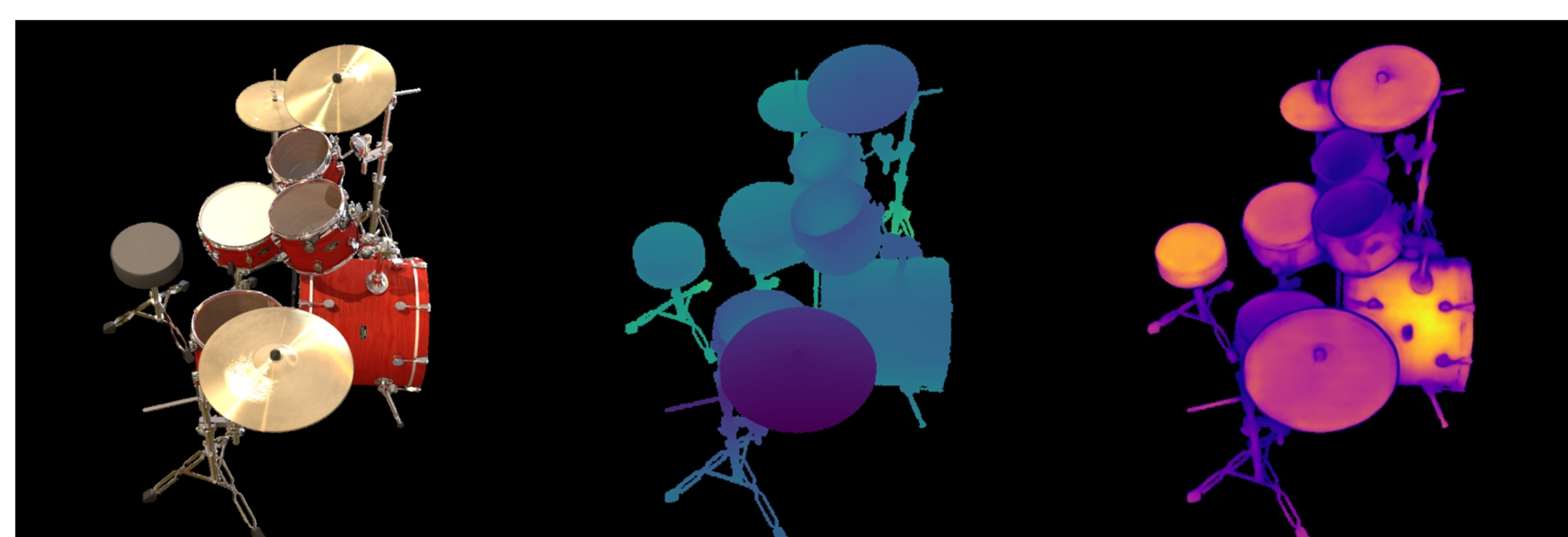
drums: VGGT | voxels | num_points=87000 Original | Depth (max=1.20) | Confidence (max=303.06)
