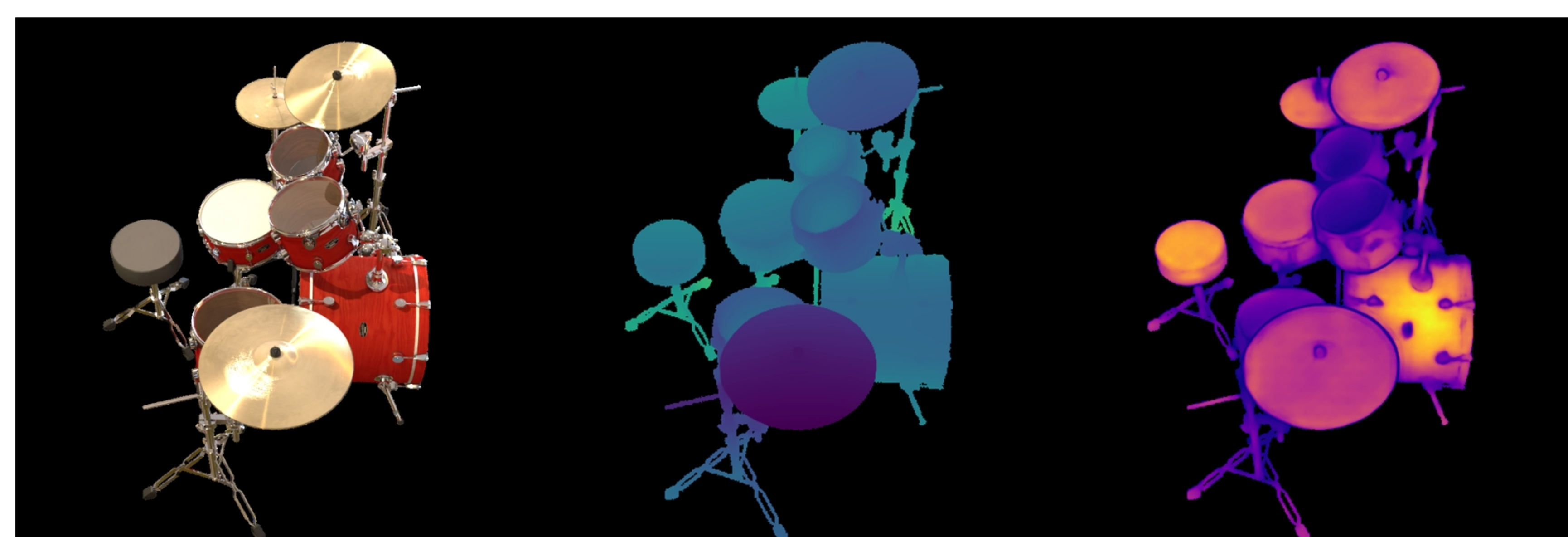
drums: VGGT | confidence | num_points=87000 Original | Depth (max=1.20) | Confidence (max=303.06)
