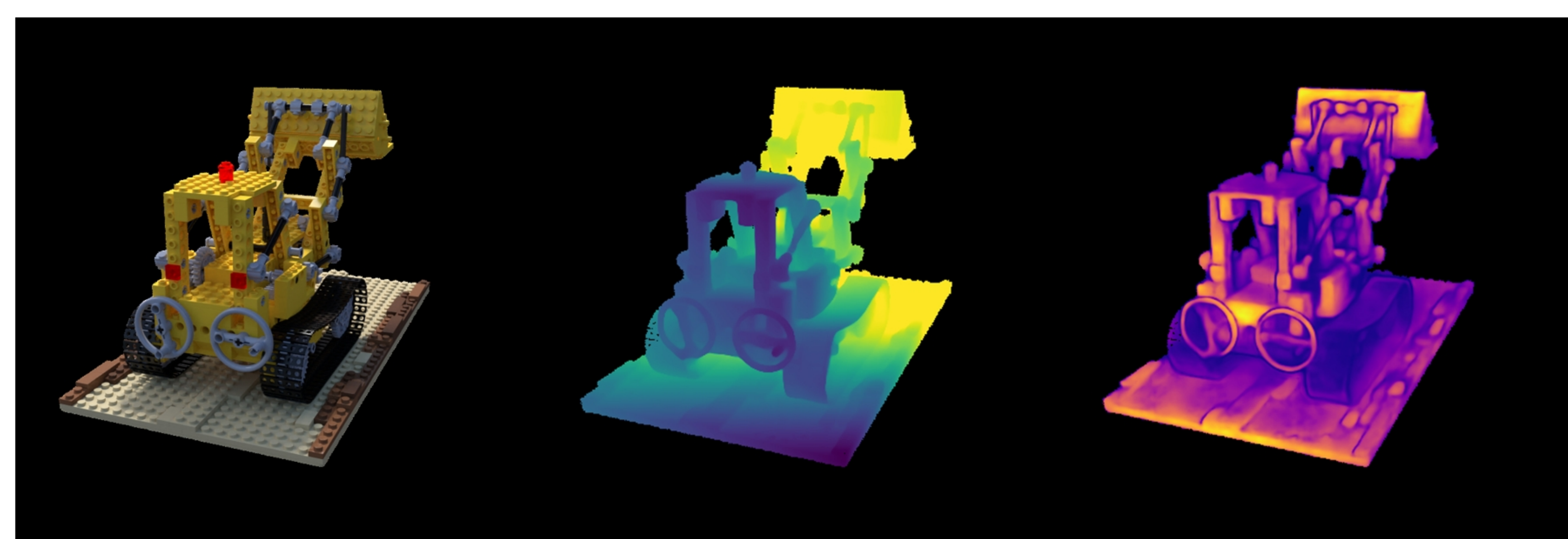
lego: VGGT | confidence | num_points=87000 Original | Depth (max=1.28) | Confidence (max=155.74)
